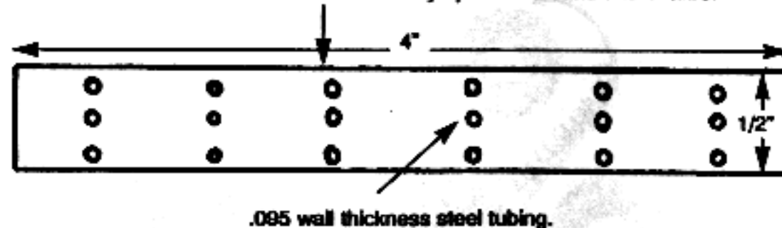
FIGURE 8 17" tube (1 1/8" O.D.).
