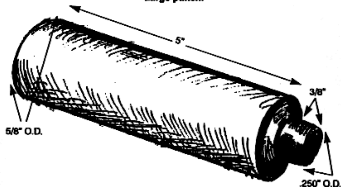
FIGURE 27 Large punch.
