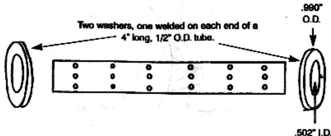
FIGURE 7 Expansion chamber.
