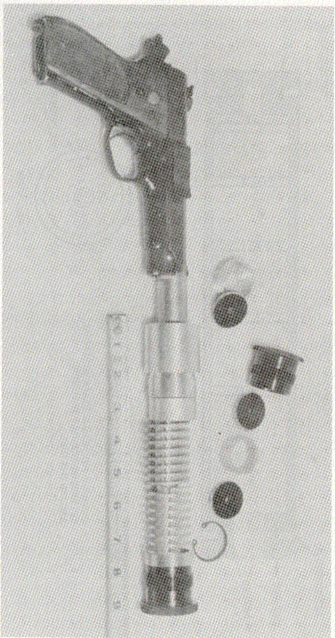
Here is a stripped silencer from a kit designed in the 1980s by RFP, Inc. Mounted on an S&W 39, this silencer is a wipe design using baffles, chambers, and an unusual ported swirl section. (Photo courtesy of J. David Truby, Silencers in the 1980s )
