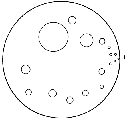
Figure V.1. The hyperbolicly congruent discs \Delta_n .
