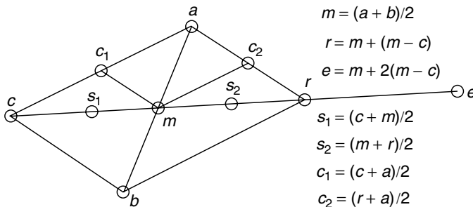
Figure 7.3 Notation used in the Nelder–Mead method.
