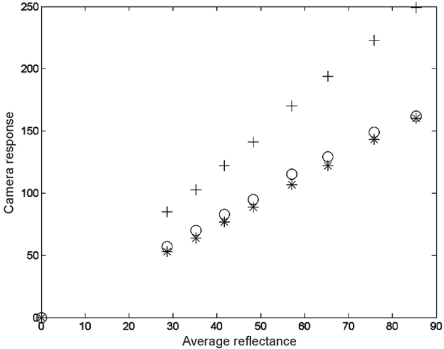
Figure 8.1 Measured camera response for red (*), green (+) and blue (○) channels for neutral ColorChecker patches of known reflectance
