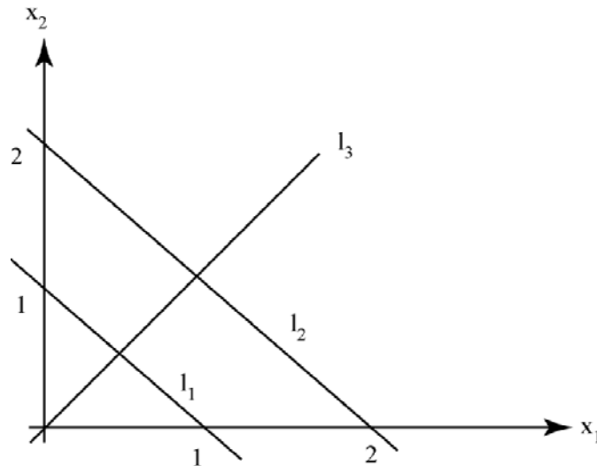
Figure 2.1.1: Infinite or None or One Solution(s)
