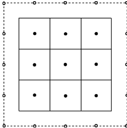
Figure 5.2.1: Grid with Artificial Grid Points
