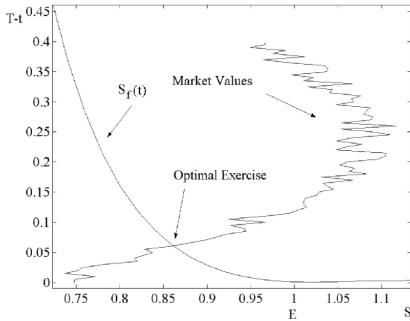
Figure 5.5.4: Optimal Exercise of an American Put
