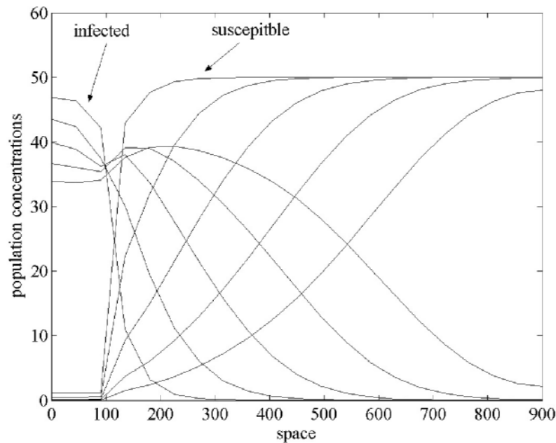
Figure 5.1.1: Infected and Susceptible versus Space
