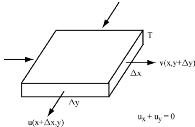
Figure 3.3.1: Incompressible 2D Fluid
