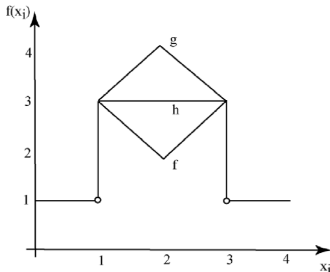
Figure 5.3.1: Three Curves with Jumps
