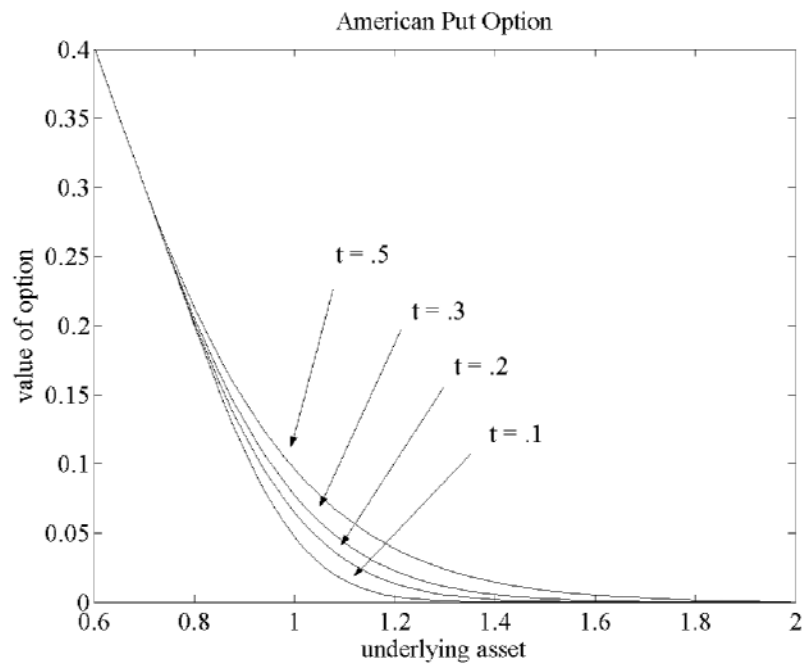
Figure 5.5.2: P(S, T-t) for Variable Times
