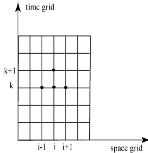
Figure 1.2.2: Time-Space Grid
