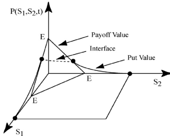
Figure 5.6.1: American Put with Two Assets
