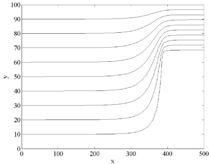
Figure 3.4.3: Flow Around an Obstacle
