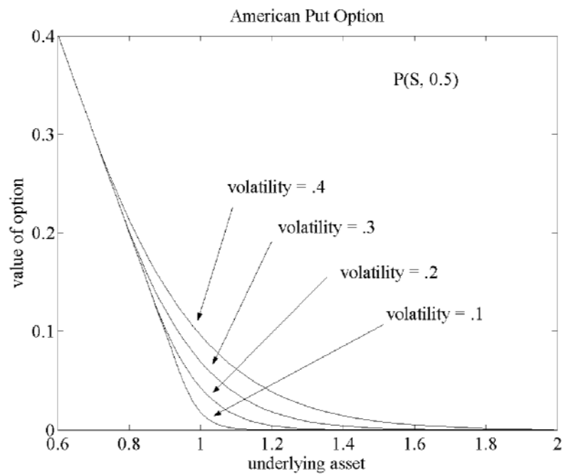
Figure 5.5.3: Option Values for Variable Volatilities
