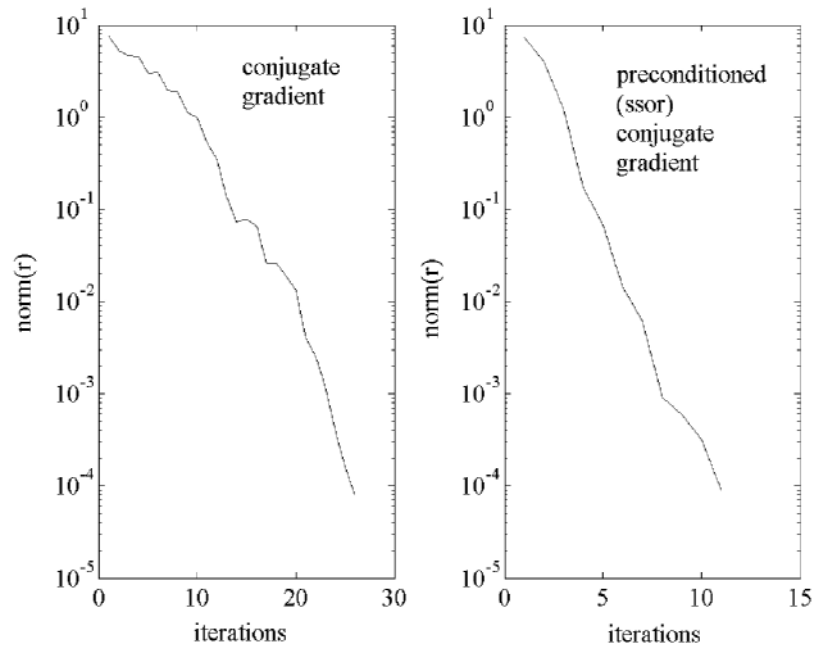
Figure 3.6.1: Convergence for CG and PCG
