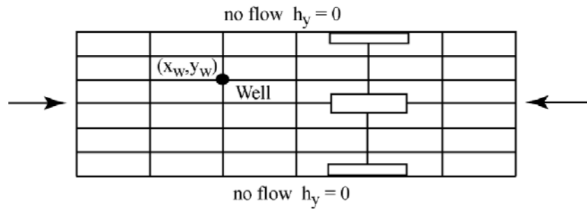
Figure 3.3.2: Groundwater 2D Porous Flow
