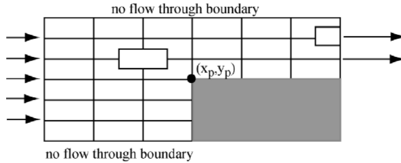
Figure 3.4.1: Ideal Flow About an Obstacle
