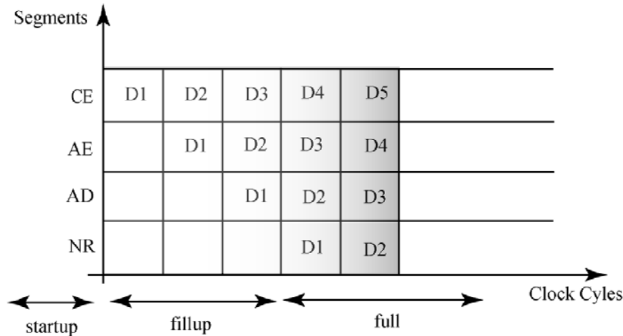
Figure 6.1.5: Vector Pipeline for Floating Point Add
