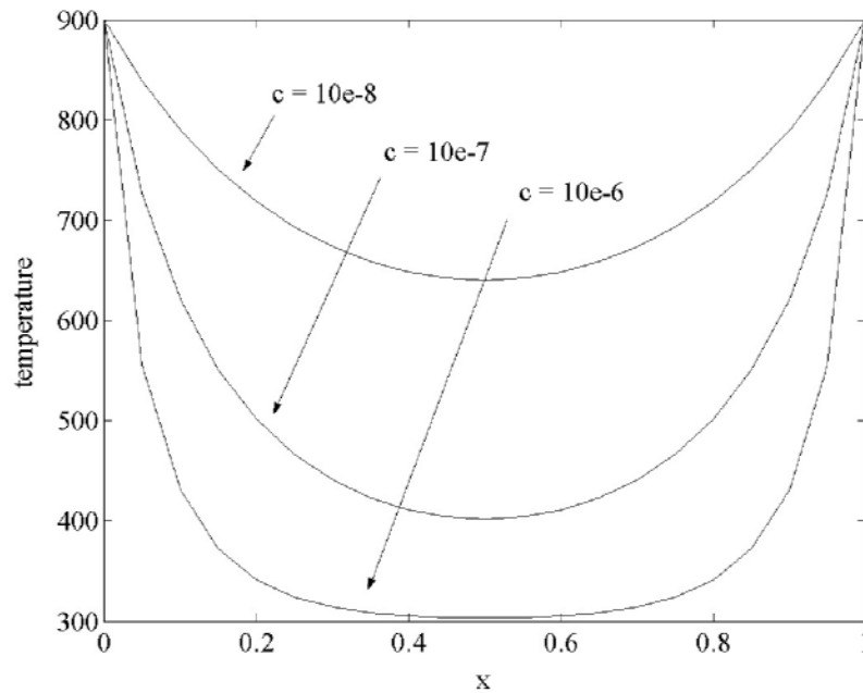
Figure 4.2.2: Temperatures for Variable c
