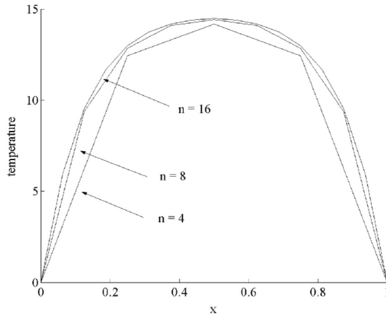
Figure 2.6.2: Variable n = 4, 8 and 16
