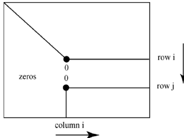
Figure 2.2.1: Gaussian Elimination
