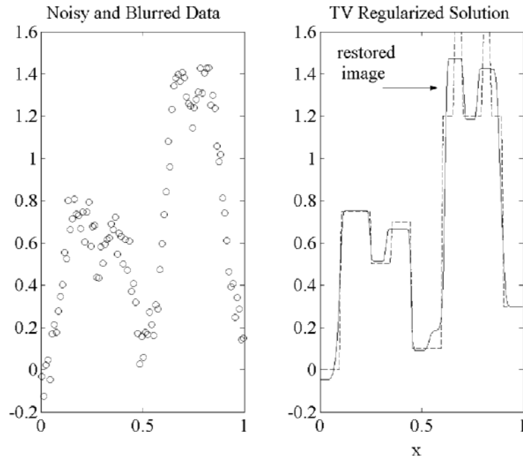
Figure 5.3.2: Restored 1D Image
