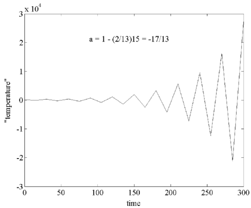
Figure 1.1.3: Unstable Computation
