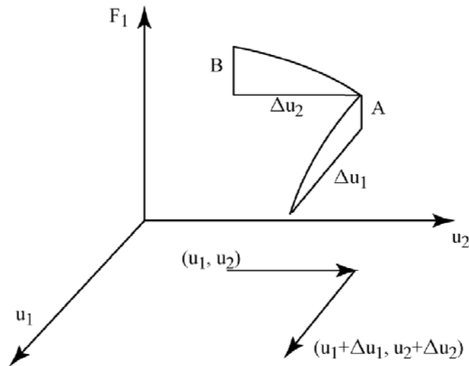
Figure 4.2.1: Change in F_1
