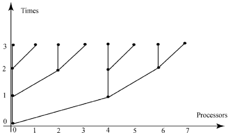
Figure 6.4.1: Fan-out Communication
