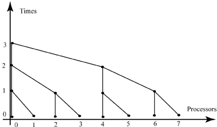
Figure 7.2.1: A Fan-in Communication
