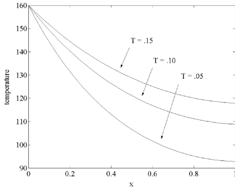
Figure 3.1.1: Cooling Fin with T = .05, .10 and .15
