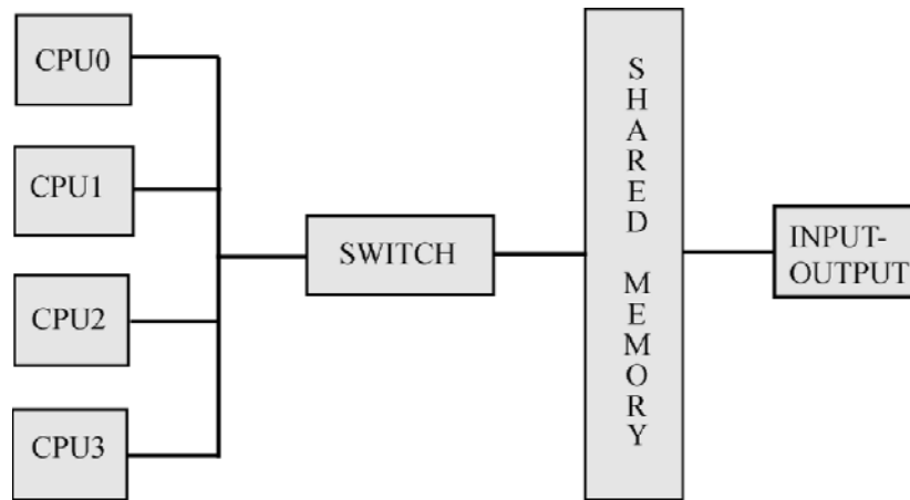
Figure 6.1.2: Shared Memory Multiprocessor
