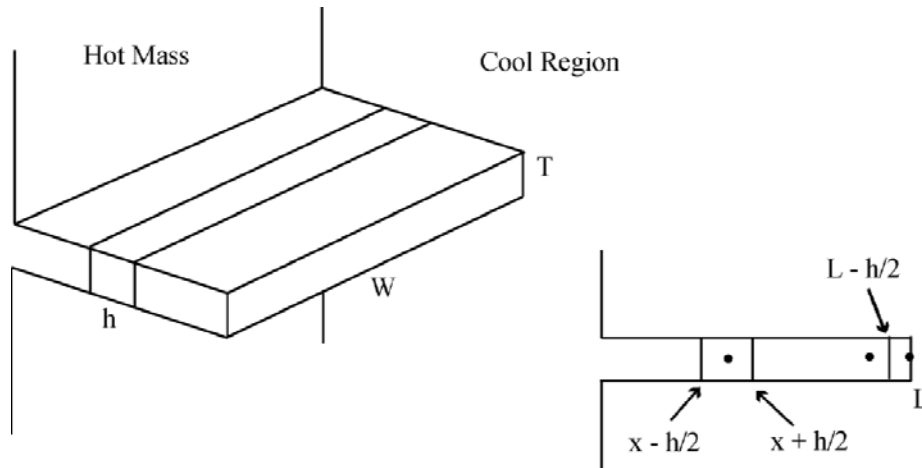
Figure 2.3.1: Thin Cooling Fin
