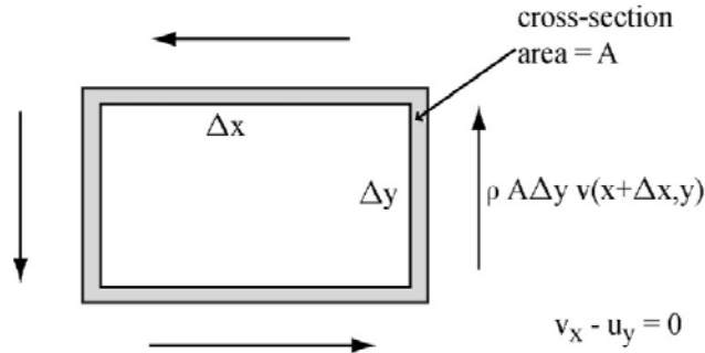
Figure 3.4.2: Irrotational 2D Flow v_x - u_y = 0
