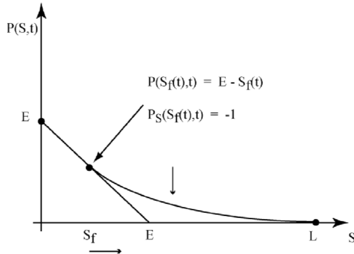
Figure 5.5.1: Value of American Put Option
