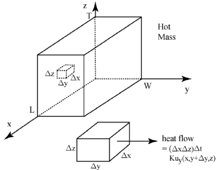
Figure 4.4.1: Heat Diffusion in 3D
