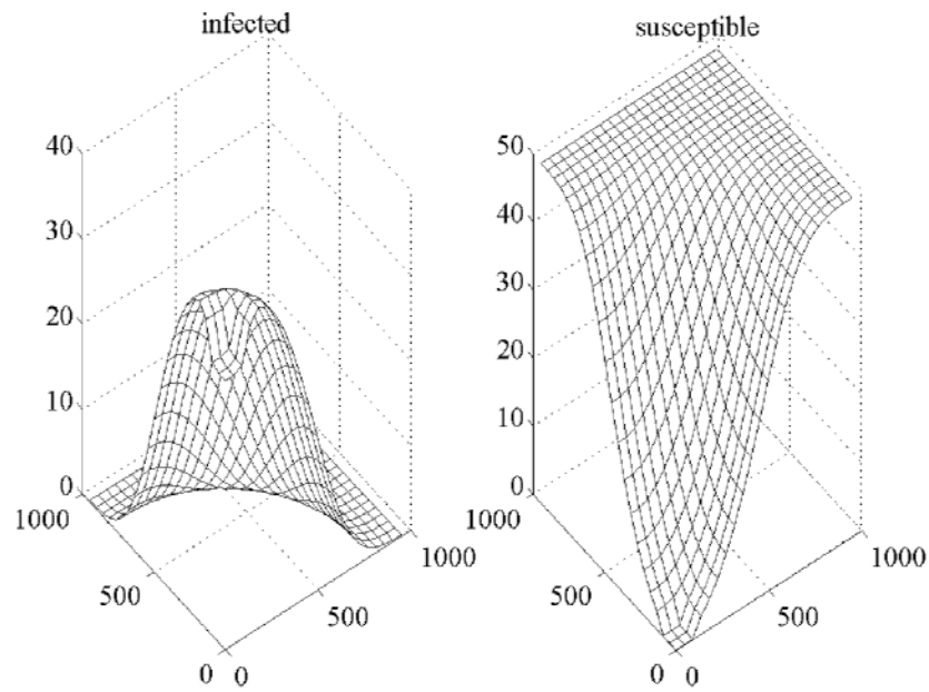
Figure 5.2.2: Infected and Susceptible at Time = 0.3
