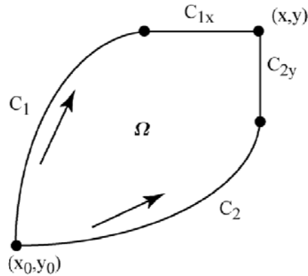
Figure 3.4.4: Two Paths to (x,y)
