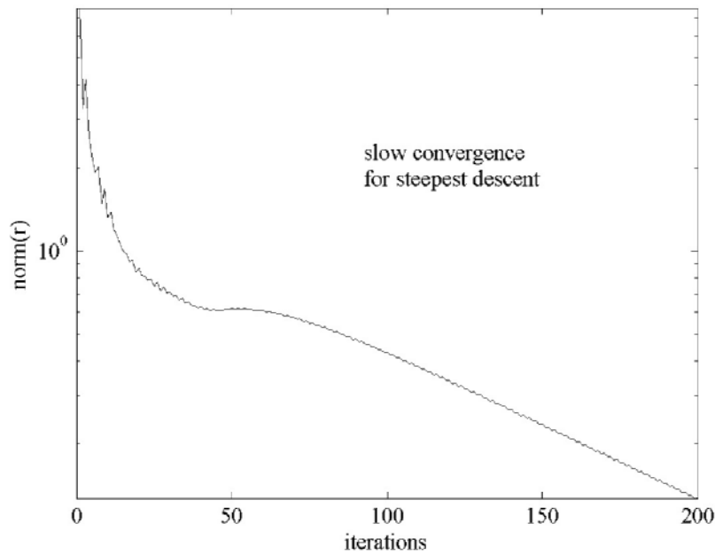
Figure 3.5.1: Steepest Descent norm(r)
