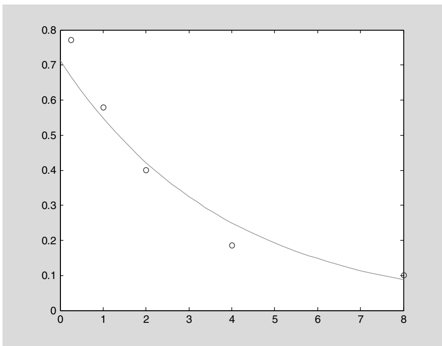
Fig. 10.4. Exponential fit for example batch experiment
