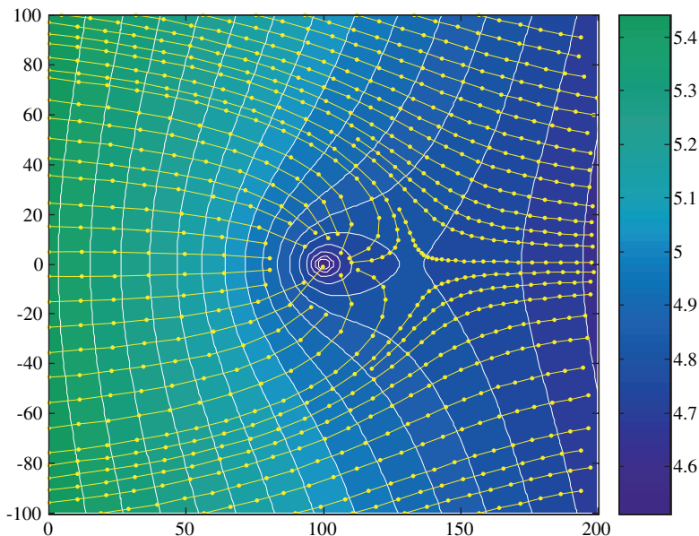
Fig. 14.6. Flow towards a well, depicted by filled head contours and flowpaths with speed dots
