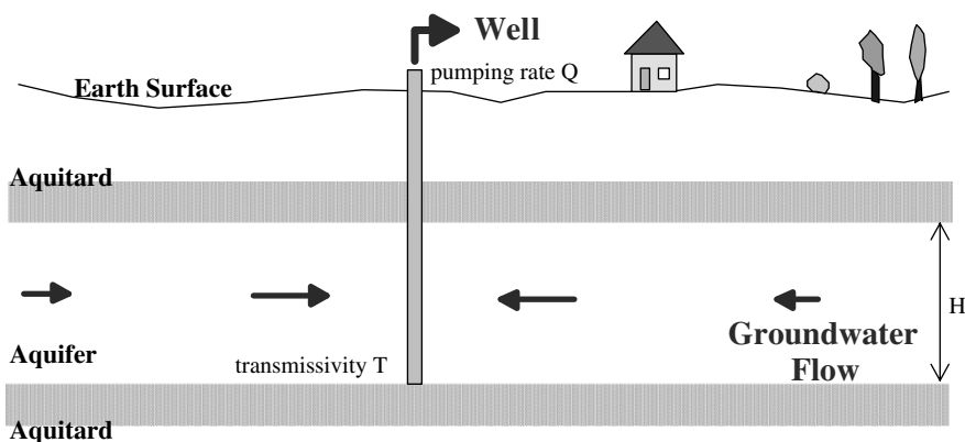
Fig. 12.1. Schematic cross-sectional view of a well pumping from a confined aquifer
