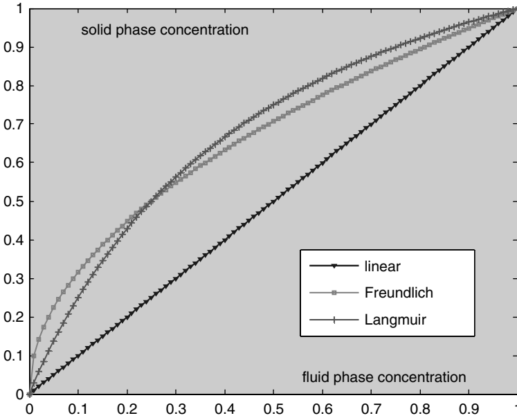
Fig. 6.2. Illustration of sorption isotherms: linear, Freundlich and Langmuir 33
