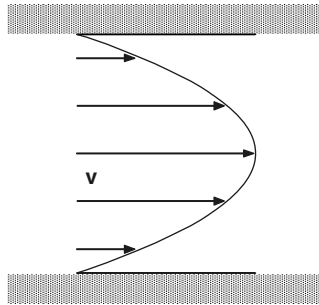
Fig. 11.3: Laminar flow between two plates
