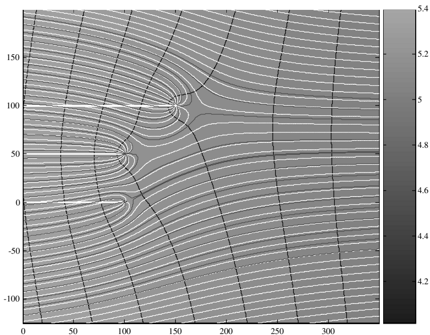
Fig. 15.2. Groundwater flow towards three wells (isopotential, streamlines and flowpaths)
