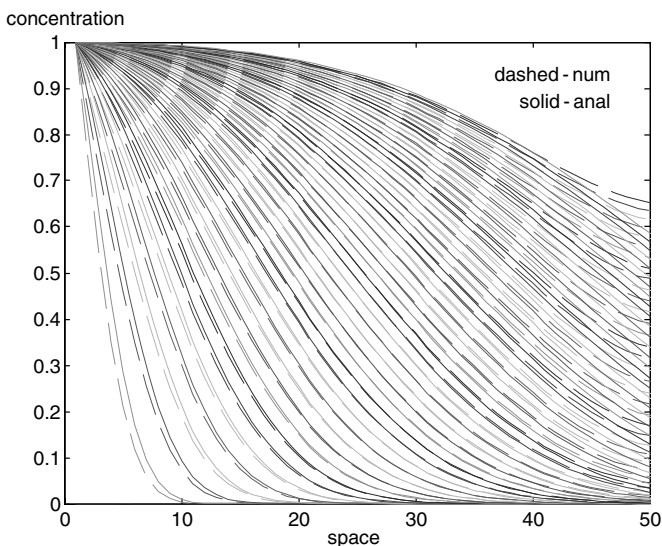
Fig. 4.9. Comparison of analytical and numerical results for the 1D transport equation
