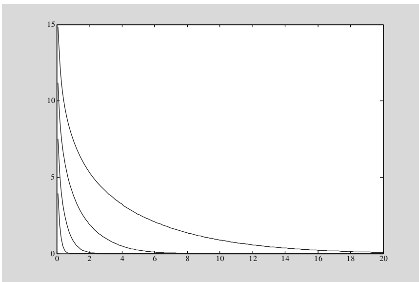
Fig. 12.7. Unsteady drawdown of groundwater piezometric head in a confined aquifer due to pumping according to Theis; parameters given in text, for times t = 10^3, 10^4, 10^5 and 10^6
