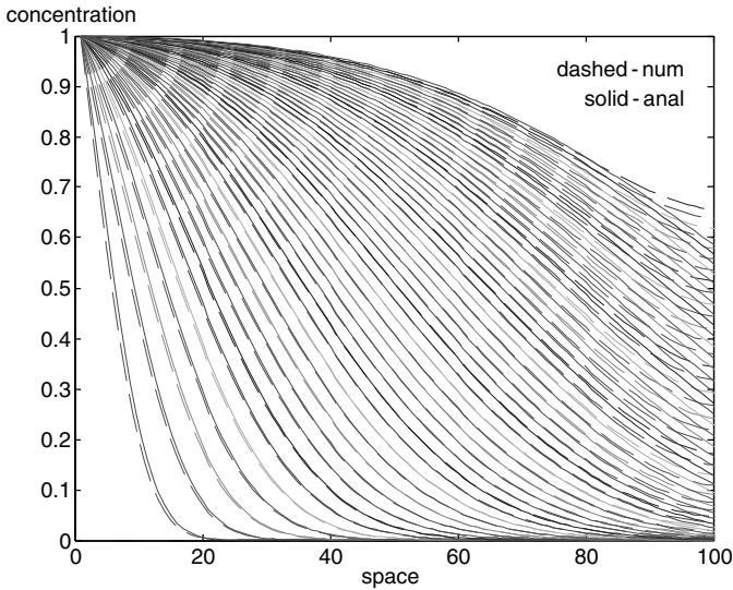
Fig. 4.10. Comparison of analytical and numerical results for the 1D transport equation, for a finer discretization
