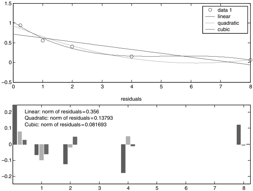
Fig. 10.3. Results for the example fitting problem, using the ‘Basic Fitting’ tool under MATLAB®
