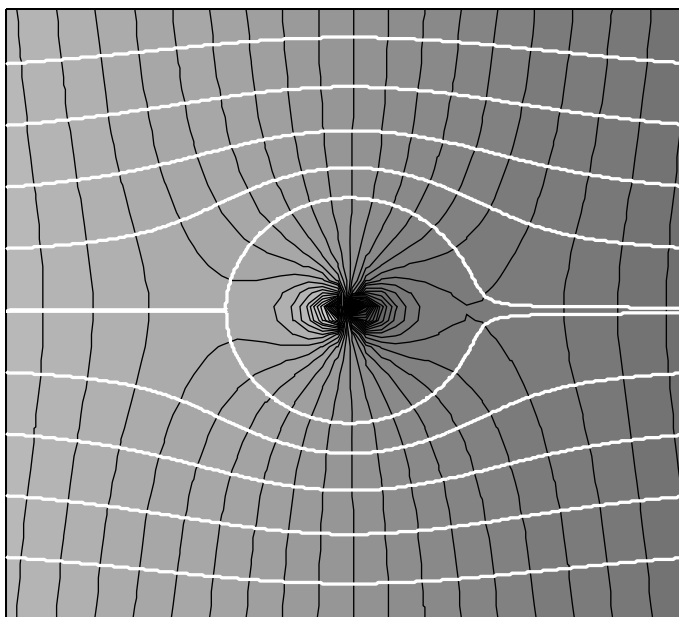
Fig. 15.9. Flow round an obstacle; groundwater flow towards a lake
