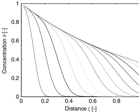
Fig. 5.6. Steady and transient solution for transport equation with degradation; dimensionless space variable \xi and dimensionless concentration \theta for Pe = 100 and Da_2 = 1
