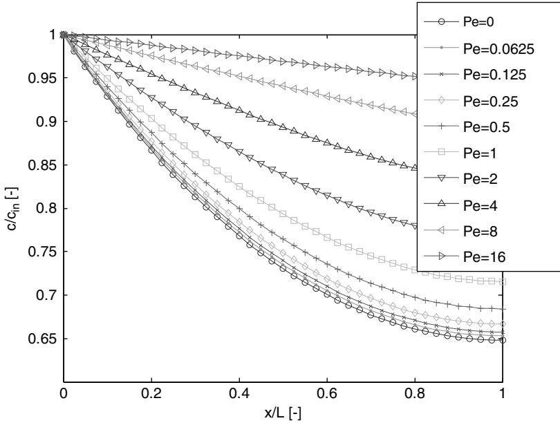
Fig. 5.5. Profiles for fluid phase concentration in case of transport with constant parameters for 2 nd Damköhler number Da_2 = 1 in dependence of the Pe
