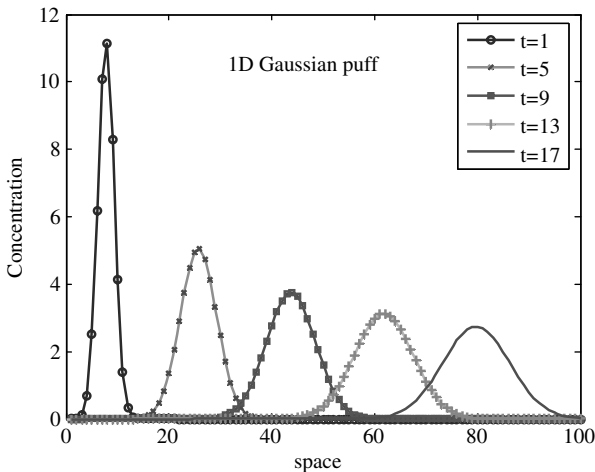
Fig. 16.1. 1D Transport solution for instantaneous source for 5 time instants
