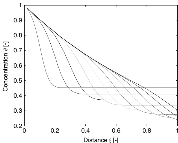
Fig. 5.7. Transient solution for transport equation with degradation; dimensionless space variable \xi and dimensionless concentration \theta for Pe = 100 and Da_2 = 1 , for c_0 = c_{in}/2 = 0.5
