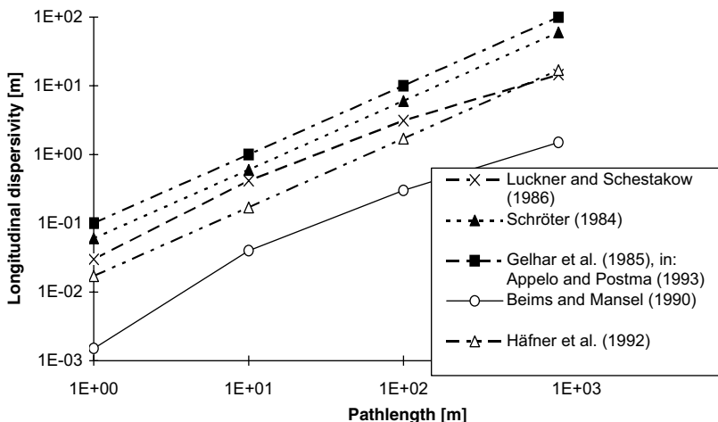
Fig. 3.3. Scale dependency of longitudinal dispersivity in porous media, as observed by different authors
