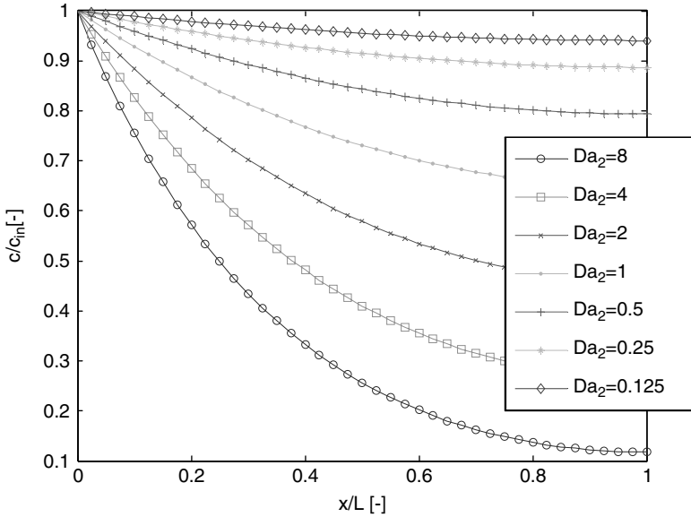
Fig. 5.2. Concentration profiles in the case of diffusion and decay with constant parameters D and \lambda ; as function of dimensionless 2 nd Damköhler number Da_2
