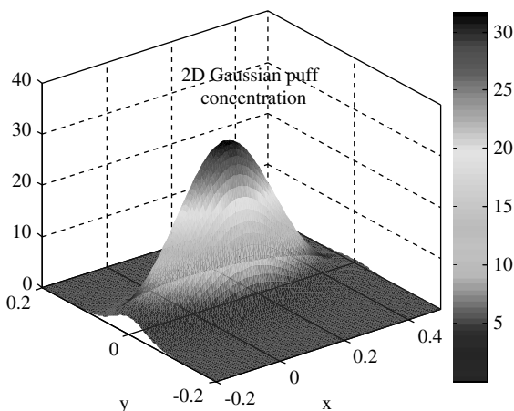
Fig. 16.4. Transport solution for an instantaneous source in 2D
