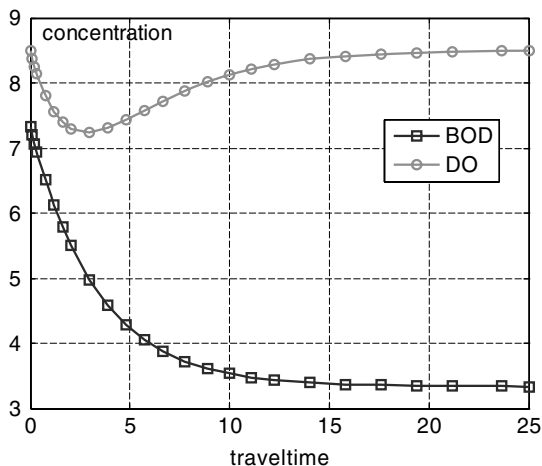
Fig. 9.1. Model results for river purification
