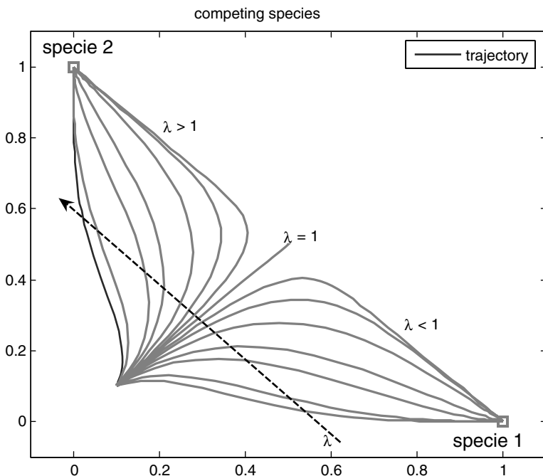
Fig. 19.3. Trajectories in phase space for the competing species model; \lambda \in \{0.2, 0.25, 0.4, 0.5, 0.667, 0.8, 0.9, 1, 1.11, 1.25, 1.5, 2, 2.5, 4, 5\} ; use the corresponding M-file for other input values
