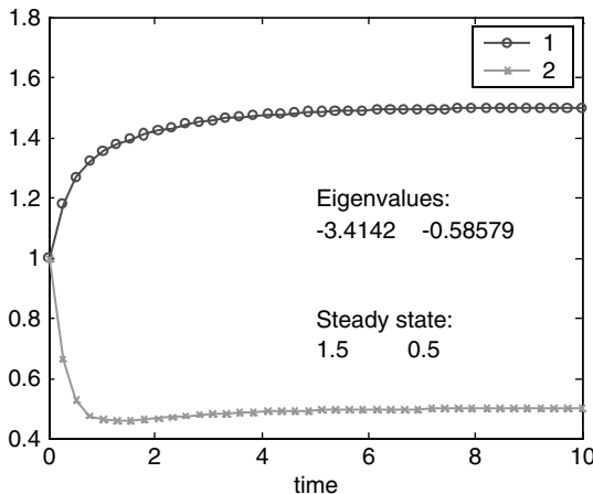
Fig. 18.7. Transient and steady state solution of a 2-compartment model using MATLAB®
