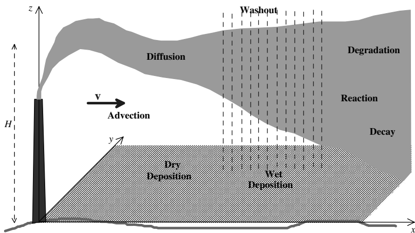
Fig. 16.6. Release from a stack; schematic illustration of parameters and processes
