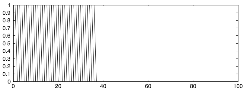
Fig. 4.4. Pure advective passing of a concentration front through a 1D compartment
