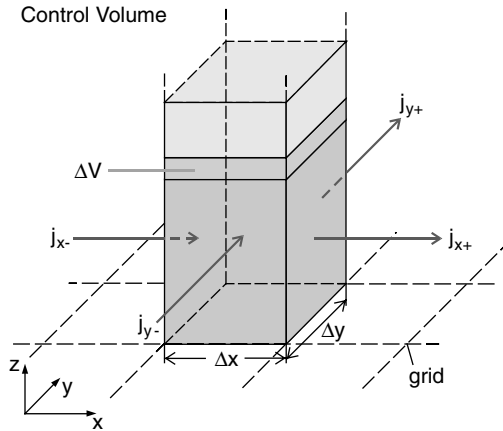
Fig. 2.4. Illustration of a control volume in two space dimensions x and y
