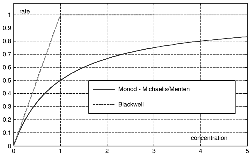
Fig. 7.1. Monod – Michaelis/Menten and Blackwell kinetics (normalized)
