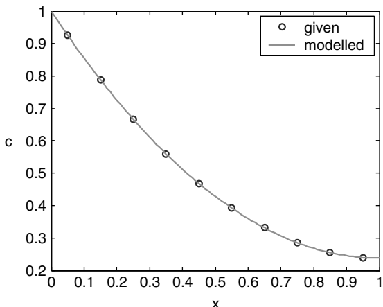
Fig. 10.8. Optimal fit for diffusivity estimation example problem
