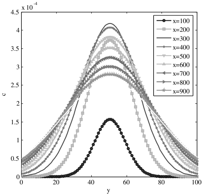
Fig. 16.8. Concentration distribution at ground surface according to a Gaussian plume; concentration at cross-sections, parallel to y -axis at various distances from the source
