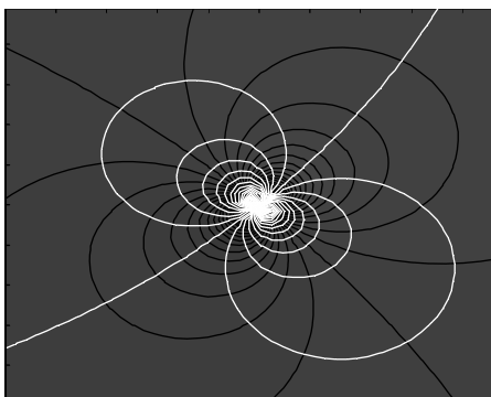
Fig. 15.8. Dipole pattern (streamlines white, potential contours black)
