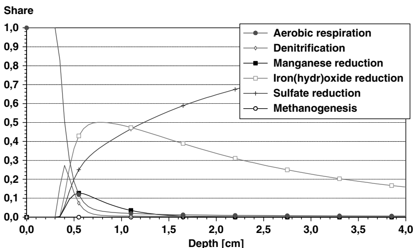
Fig. 9.4. Redox-sequence in aquatic sediments, see van Cappellen & Wang (1995, 1996); recalculated by the author
