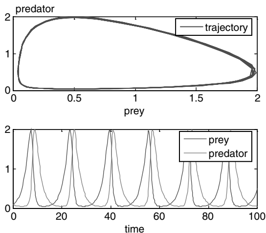
Fig. 19.5. Example output of a predator-prey model
