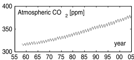
Fig. S.4. Atmospheric CO 2 increase; visualized using MATLAB®
