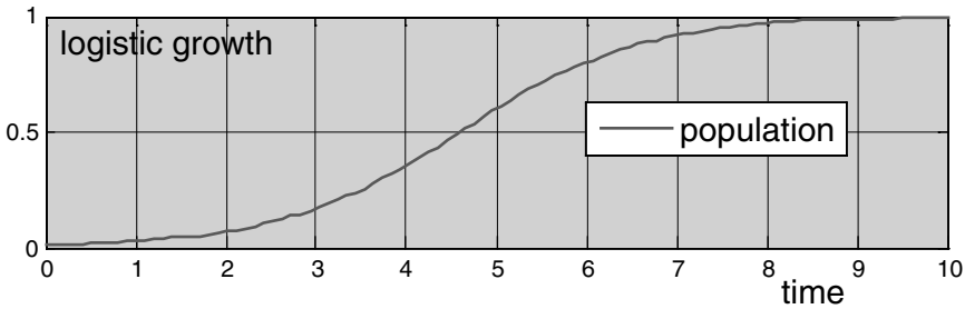
Fig. 19.1. Logistic growth; computed from analytical solution using MATLAB®
