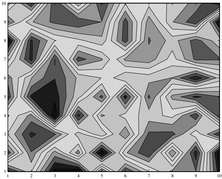
Fig. 13.5. Surface plot and filled contours for a matrix
