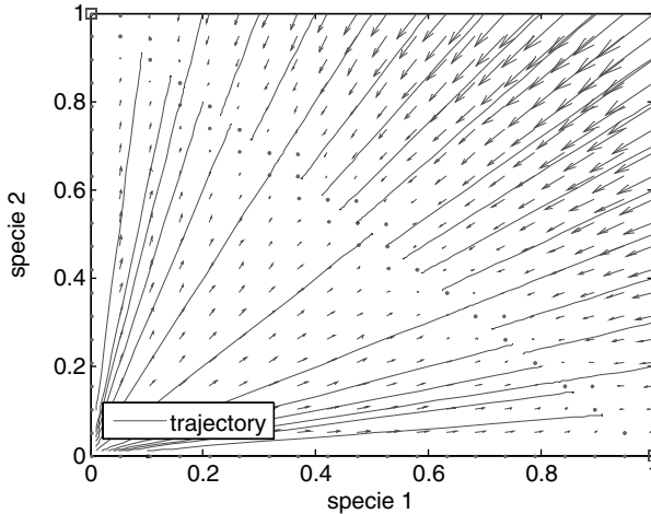
Fig. 19.4. Trajectories in the phase space for the degenerate case \lambda = 0 of the competing species model; all equilibria on the diagonal line (from upper left to lower right) are stable
