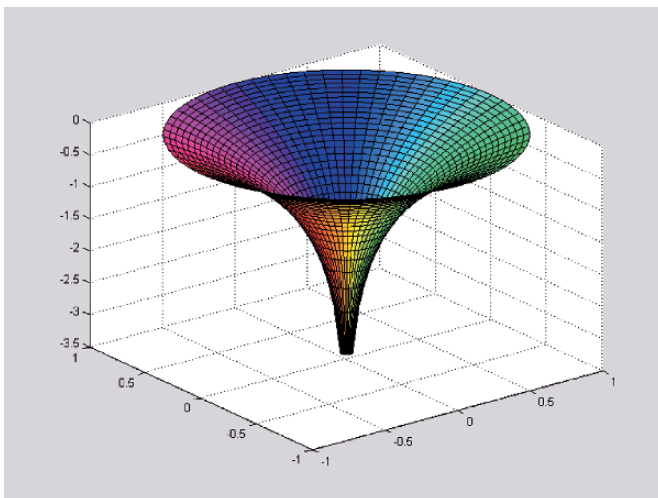
Fig. 15.7. Surface plot of the complex logarithm
