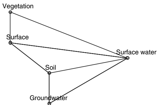
Fig. 18.3. Graph, representing a flux network between compartments, visualized using MATLAB®
