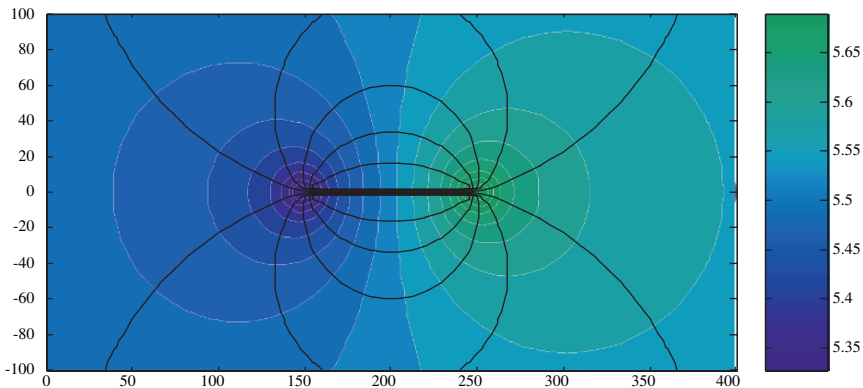
Fig. 15.3. Doublette system (isopotential and streamlines)
