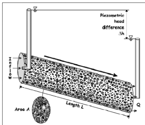
Fig. 11.7. Typical set-up of a Darcy-experiment; for examination of Darcy's Law and the determination of hydraulic conductivity
