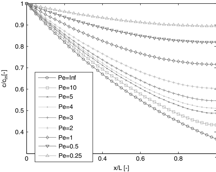
Fig. 5.3. Profiles for fluid phase concentration in case of transport with constant parameters for Da_1 = 1 in dependence of the Péclet number Pe
