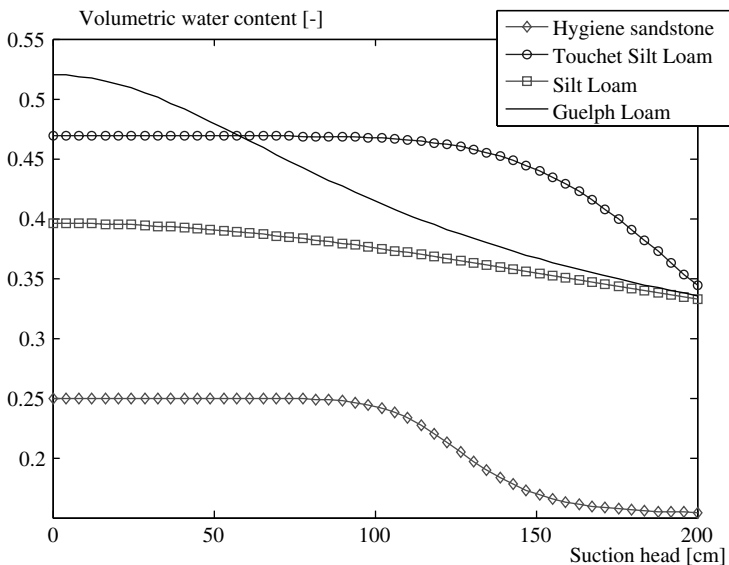
Fig. 11.8. Examples of retention curves, data from Hornberger & Wiberg (2005); produced using MATLAB®
