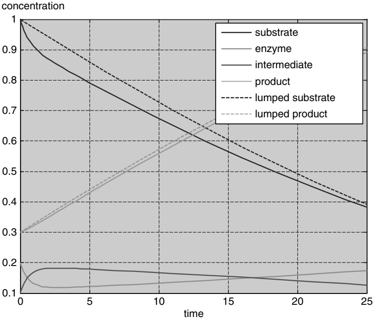
Fig. 9.2. Comparison of a detailed 4-species model and the approximation using Michaelis-Menten kinetics
