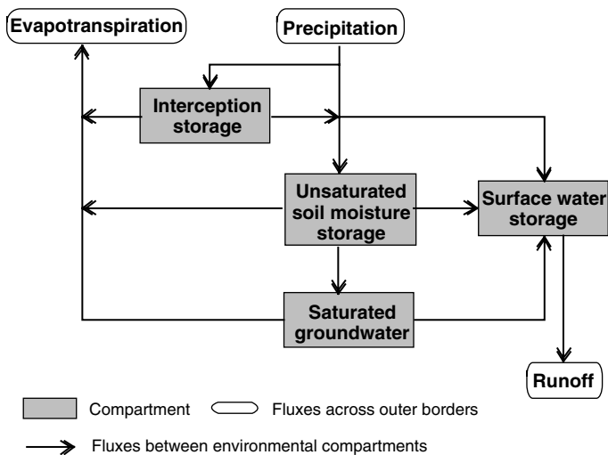
Fig. 18.1. Network of compartments for modeling the terrestrial part of the hydrological cycle according to Freeze & Cherry (1979), modified by E.H
