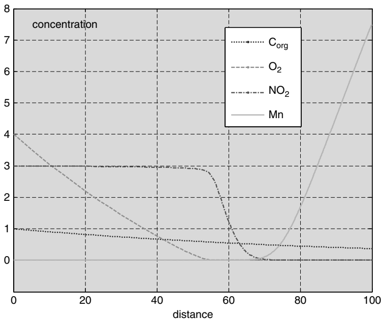
Fig. 9.5. Result of MATLAB® example for the redox sequence example
