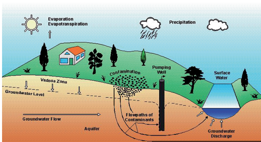
Fig. 11.6. Crucial sub-surface flow paths at waste disposal sites
