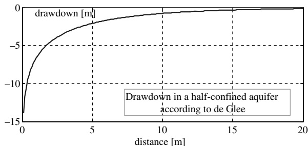
Fig. 12.5. Drawdown of groundwater piezometric head in a half-confined aquifer due to pumping, according to de Glee (1930)
