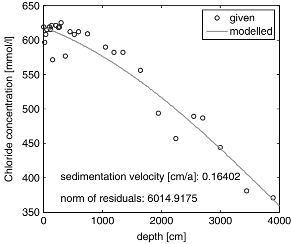
Fig. 10.7. Exponential fit for \lambda and c_0
