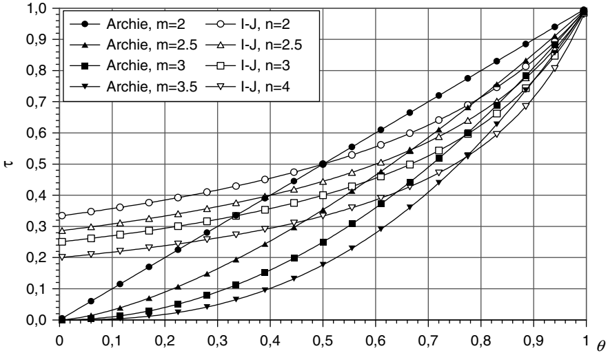
Fig. 3.2. Tortuosity \tau as function of porosity \theta , according to Archie's Law for different values of parameter m , and according to Iversen & Jørgensen (I-J) for parameter values of n
