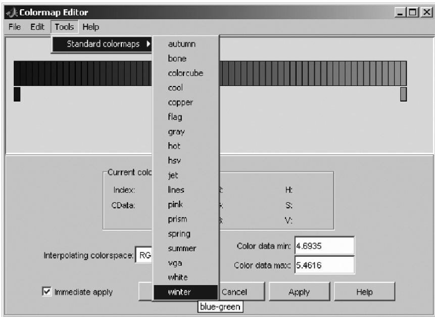
Fig. 14.4. Colormap editor
