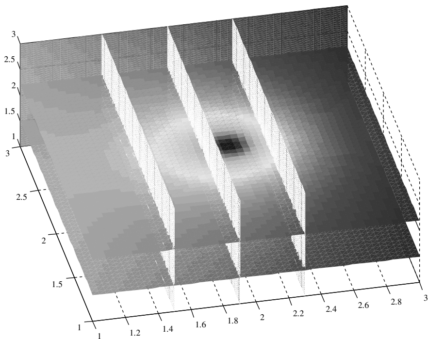
Fig. 14.2. Potential flow in 3D
