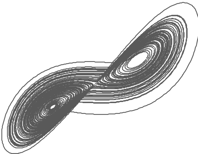
Fig. 19.7. The Lorenz attractor, produced using MATLAB®
