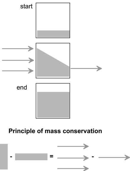
Fig. 2.3. Illustration for the derivation of the mass conservation equation
