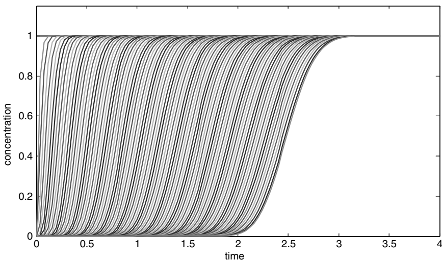
Fig. 4.11. Breakthrough curves as result of the transport solution using MATLAB® pdepe
