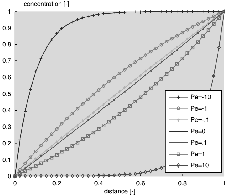
Fig. 9.3. The steady-state solution of the advection-diffusion equation in dimensionless form in dependence of the dimensionless Péclet number
