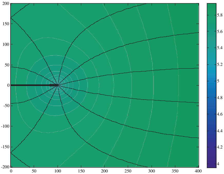
Fig. 15.5. Bank filtration example plot (for x_0 = 100 m, Q_{x_0} = -10^{-6} m 2 /s, Q = 0.001164 m 3 /s)
