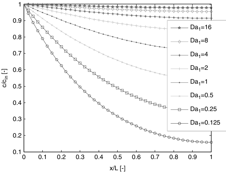
Fig. 5.4. Profiles for fluid phase concentration in case of transport with constant parameters for Pe = 1 in dependence of the 1 st Damköhler number Da_1
