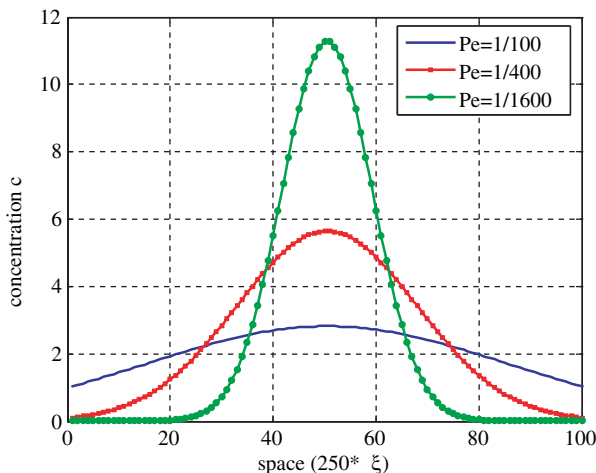
Fig. 16.2. Transport solution for instantaneous source in dependence of the Péclet number Pe
