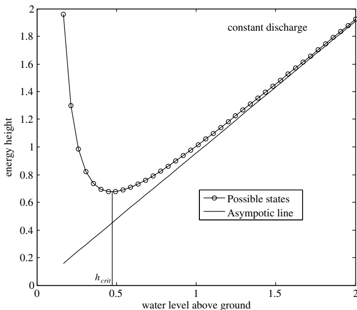
Fig. 11.5. Energy height and water level characteristic for open channel flow
