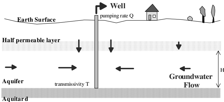
Fig. 12.4. Schematic cross-sectional view of a well pumping from a half-confined aquifer
