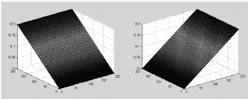
Fig. 13.4. Two examples for baseflow for confined aquifer (with reference head 10 m K = 10^{-4} m/s); left: in x -direction ( Q_{x0} = -10^{-6} , Q_{y0} = 0 ), right: in y -direction ( Q_{x0} = 0 , Q_{y0} = -10^{-6} )
