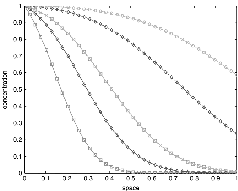
Fig. 6.3. Result of exercise 6.1; both situations are represented by three concentration distribution diagrams. Squares mark t=1/3 , diamonds t=2/3 and circles t=1 . The graph for R=1 and t=1/3 falls together with the graph for R=3 and t=1
