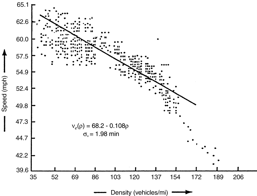
Fig. 5.9 Speed–density relationship.
