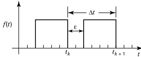
Fig. 7.15 DVM gating waveform.
