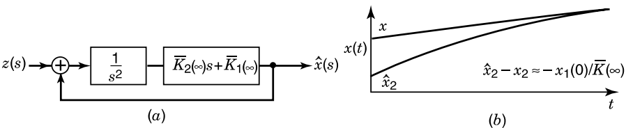
Fig. 7.10 Type 2 servo (a) and servo estimates (b).
