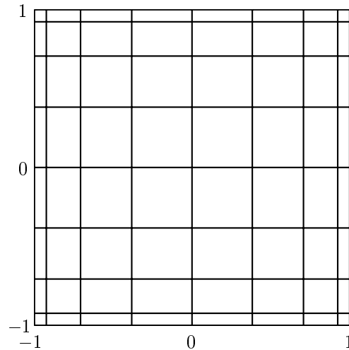
Fig. 7.1. A tensor product grid.
