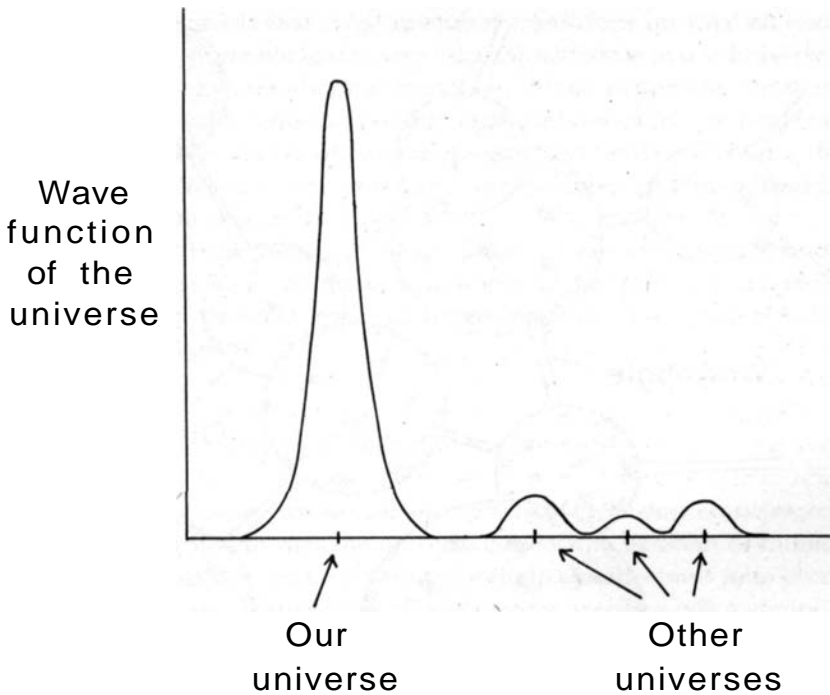
Figure 12.1. In Hawking's wave function of the universe, the wave function is most likely concentrated around own universe. We live in our universe because it is the most likely, with the largest probability. However, there is a small but non-vanishing probability that the wave function prefers neighboring, parallel universes. Thus transitions between universes may be possible (although with very low probability).
