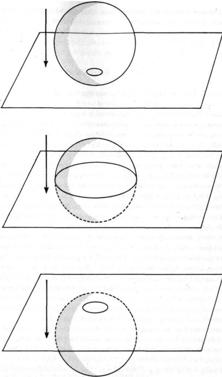
Figure 3.1. In Flatland, Mr. Square encounters Lord Sphere. As Lord Sphere passes through Flatland, he appears to be a circle that becomes successively larger and then smaller. Thus Flatlanders cannot visualize three-dimensional beings, but can understand their cross sections.
