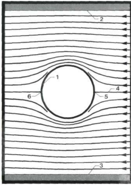
(b) Streamlines
