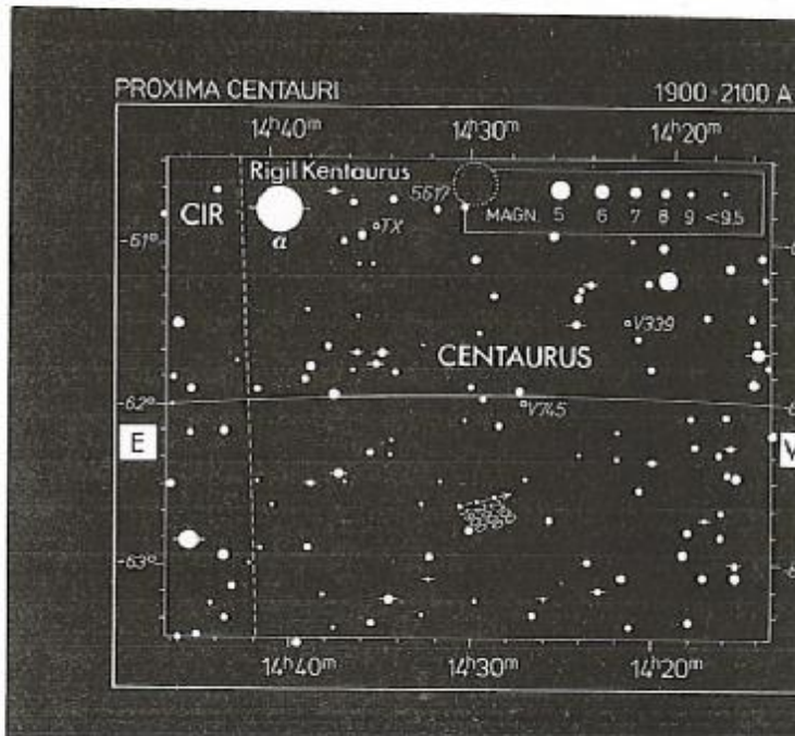
Fig. 93. A chart showing the region near Proxima Centauri, the nearest star to the sun. Because it is so close, over a period of years it moves with respect to more distant stars, as marked. (W
