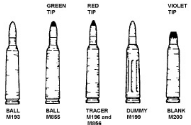
Figure 2-14. Authorized Ammunition.
