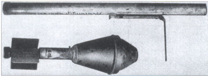
The Panzerfaust 30 is depicted here with its warhead removed. The thin sheet metal fins 'unwrapped' when the warhead was launched. While it is similar in appearance to the Panzerfaust 60, the folding sights are of distinctly different design.
