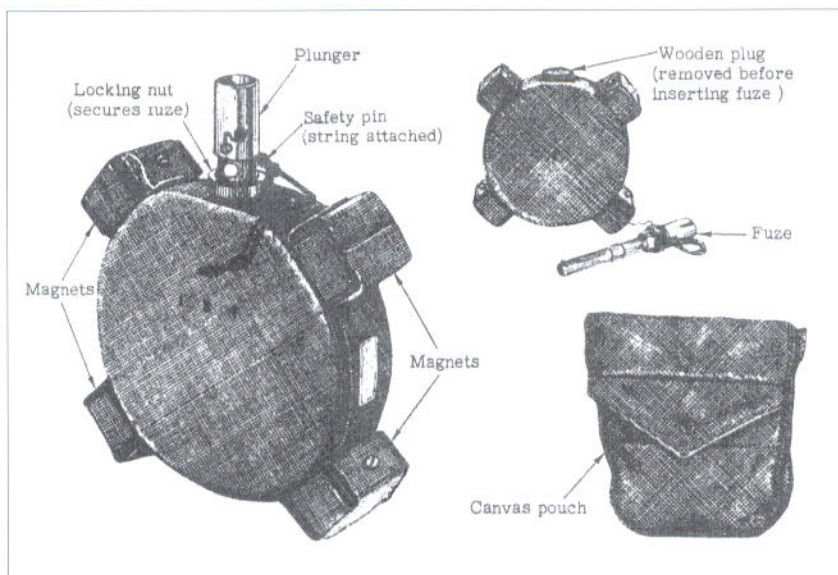
The Japanese Type 99 (1939) AT charge (99 hako-bakurai) was small (about 4 3 / 4 in x 1 1 / 2 in without the four magnets), but if two or more could be fastened together they caused a great deal of concern to tankers (see Plate H). It was issued in a canvas carrying pouch, with the fuze packed in a two-piece metal tube under the pouch flap.
