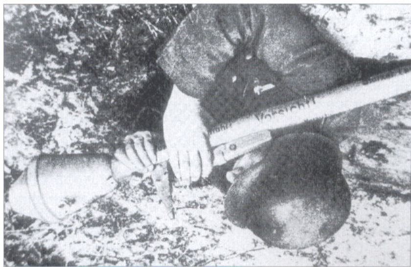
This Panzerfaust 60 was the most common of several models produced. The sight was folded down until the weapon was readied for firing. When using a Panzerfaust from a trench the firer had to be careful that the back-blast was not deflected into his confined position by a rear parapet. Most Panzerfausts were painted dark ochre yellow, but some field-grey. They were marked in red on the tube: 'Vorsicht! Starker Feuerstrahl!' ('Danger! Intense fire flash!'), with an arrowhead pointing to the rear. Operating instructions were printed on the lower portion of the projectile.
