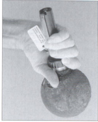
The No.68 rifle-launched AT grenade, and the 2.5in cup discharger fitted to the muzzle of an SMLE; the tin label reminds the fire to pull the safety pin before inserting it. The grenade's original paint finish is dark buff, with a red 'filling stripe' overlapping the threads of the screw-on cap, above green/black/green stripes identifying the filling as pentolite, the preferred shaped-charge explosive. (Photo Richard Hook)
