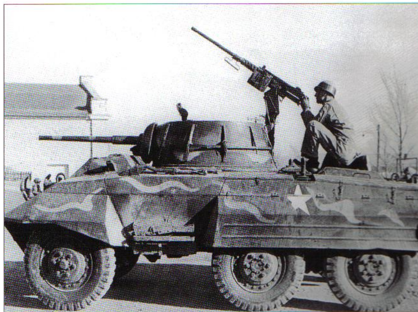
The cavalry pressed for an antiaircraft machine gun for the M8 leading to the development of the D67511 folding pintle bracket mount seen here during trials. Adopted for production because it was lighter than a ring mount, this photo clearly illustrates its main tactical drawback: if the machine gun was aimed at targets in front of the vehicle, the gunner was completely exposed on the rear deck of the vehicle. (NARA)
