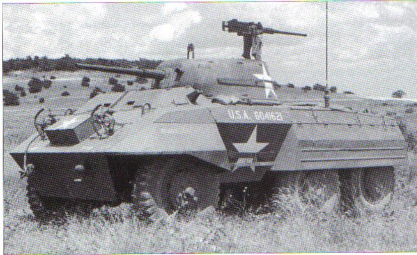
This is an example of the new production configuration in the summer of 1944 with the D67511 folding pintle bracket mount, the barrel clip on the turret roof, and the added stowage box on the glacis plate. This is from the July 1944 production run, and still retains the side mine rack which was dropped from production late in 1944. (Patton Museum)
