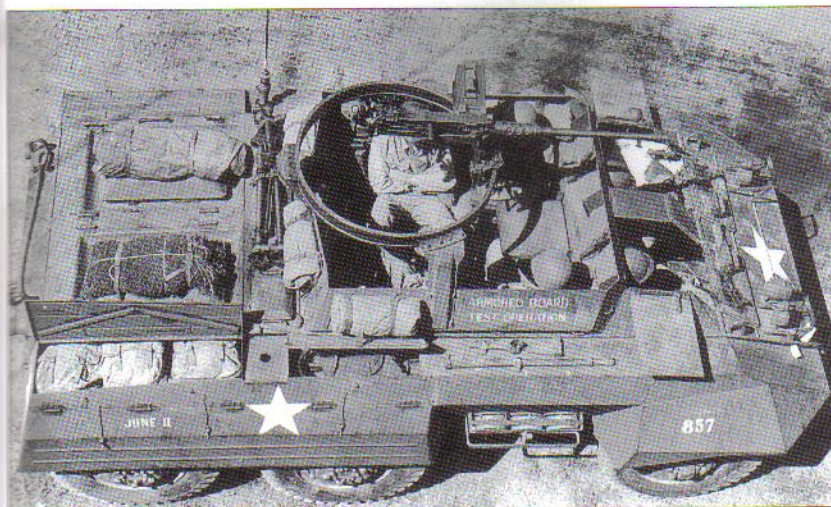
ABOVE The M20 armored utility car was a simple adaptation of the M8 armored car with the turret replaced by a simple parapet and ring mount. This photo was taken by the Armored Board at Ft. Knox in 1943 to show the proper positioning of the vehicle stowage. (NARA)
