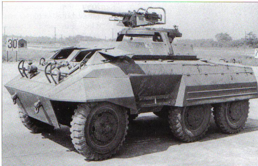
The M20 was used as a test-bed for the T86 machine gun mount, a twin .50-cal. machine gun mount adapted from the Navy's Mk 17. It was never seriously considered for use on either the M8 or M20, but the superior performance of its roller bearing construction led to the improved M66 ring mount. (NARA)
