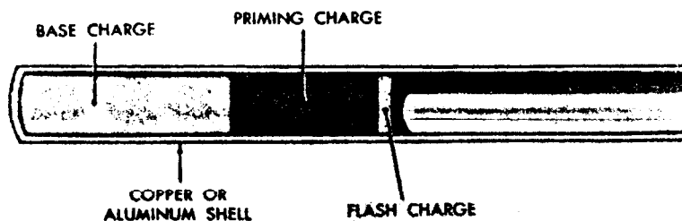
NON-ELECTRIC BLASTING CAP
