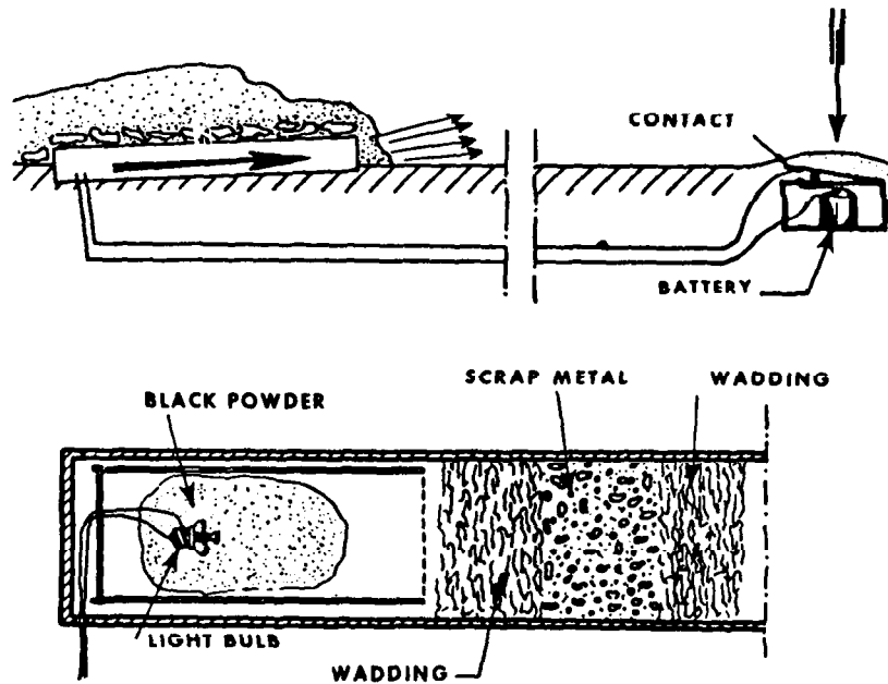
DETAIL OF EMPLACED EXPLOSIVE CHARGE
