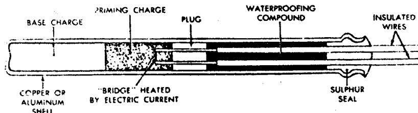
ELECTRIC BLASTING CAP
