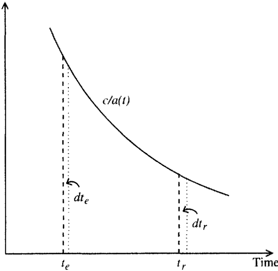
Figure A2.1 A graph of c/a(t) illustrates how the redshift law can be derived.
