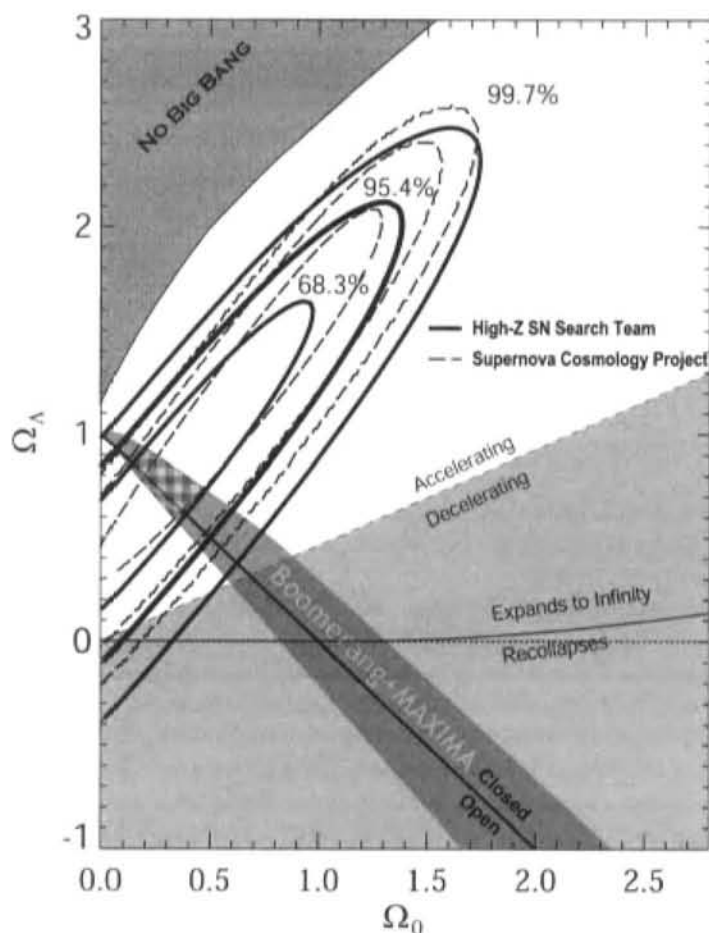
Figure A2.4 The contours show observational constraints from the supernova luminosity–redshift diagram, displayed in the \Omega_0 – \Omega_\Lambda plane as introduced in Section 7.3. Results from two separate observational programs are shown. In addition, the dark shaded region shows the part of the plane permitted by cosmic microwave background data obtained by the Boomerang and Maxima experiments, as described in Advanced Topic 5.4. Only a very small region, with \Omega_0 \simeq 0.3 and \Omega_\Lambda \simeq 0.7 , matches both data sets. [Figure courtesy Brian Schmidt.]
