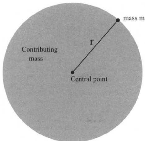
Figure 3.1 The particle at radius r only feels gravitational attraction from the shaded region. Any gravitational attraction from the material outside cancels out, according to Newton's theorem.
