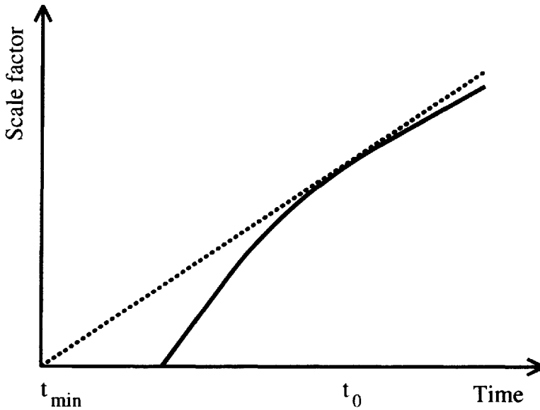
Figure 14.1 The solid line shows the true (decelerating) scale factor. The dotted line extrapolated back from the present shows the earliest possible time that the scale factor can have been zero.
