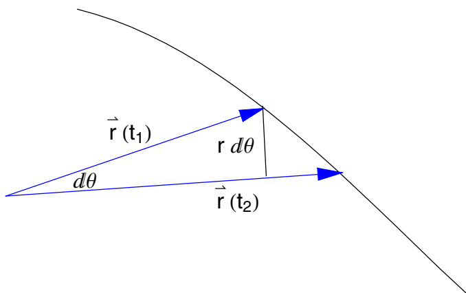
Figure 2.5.6. The position vector \vec{r} overruns in a time interval dt = t_2 - t_1 an area dA .
