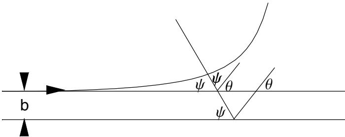
Figure 2.5.21. Angular relations between the scattering angles and the impact parameter.
