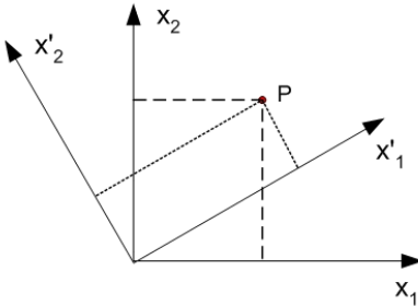
Figure 2.2.2. Rotation of the original coordinate axis.
