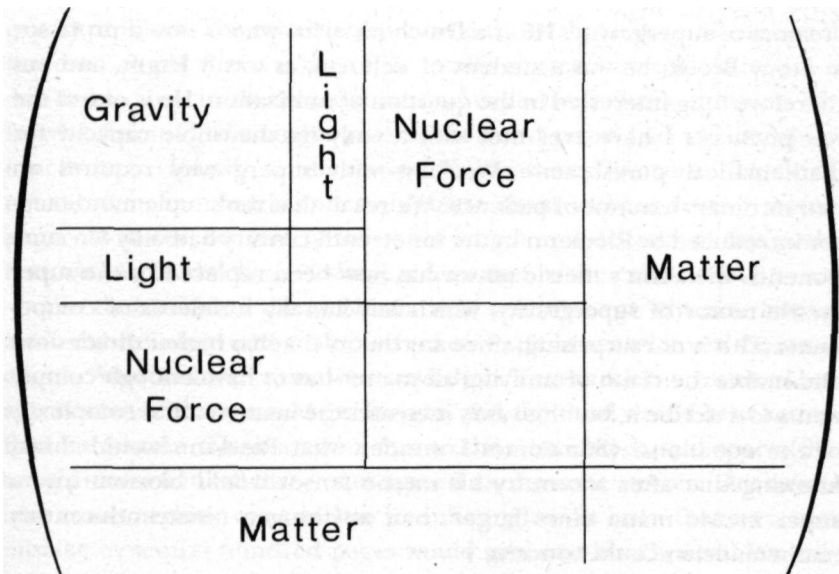
Figure 6.4. In supergravity, we almost get a unification of all the known forces (marble) with matter (wood). Like a jigsaw puzzle, they fit inside Riemann's metric tensor. This almost fulfills Einstein's dream.
