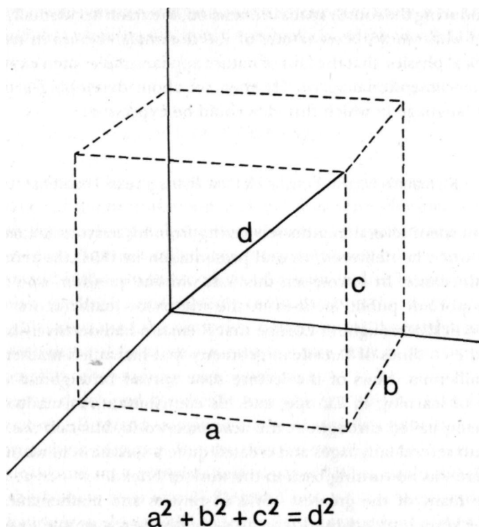
Figure 2.1. The length of a diagonal of a cube is given by a three-dimensional version of the Pythagorean Theorem: a^2 + b^2 + c^2 = d^2 . By simply adding more terms to the Pythagorean Theorem, this equation easily generalizes to the diagonal of a hypercube in N dimensions. Thus although higher dimensions cannot be visualized, it is easy to represent N dimensions mathematically.
