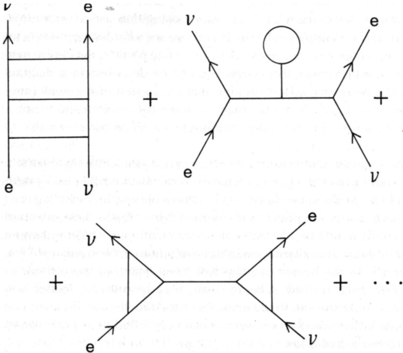
Figure 5.2. (a) In quantum theory, when subatomic particles bump into one another, they exchange packets of energy, or quanta. Electrons and neutrinos interact by exchanging a quantum of the weak force, called the W particle, (b) To calculate the complete interaction of electrons and neutrinos, we must add up an infinite series of graphs, called Feynman diagrams, where the quanta are exchanged in increasingly complicated geometric patterns. This process of adding up an infinite series of Feynman graphs is called perturbation theory.
