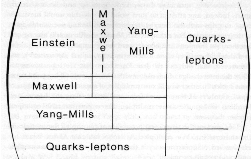
Figure 6.3. Supergravity almost fulfills Einstein's dream of giving a purely geometric derivation of all the forces and particles in the universe. To see this, notice that if we add supersymmetry to the Riemann metric tensor, the metric doubles in size, giving us the super Riemann metric. The new components of the super Riemann tensor correspond to quarks and leptons. By slicing the super Riemann tensor into its components, we find that it includes almost all the fundamental particles and forces in nature: Einstein's theory of gravity, the Yang-Mills and Maxwell fields, and the quarks and leptons. But the fact that certain particles are missing in this picture forces us to go a more powerful formalism: superstring
