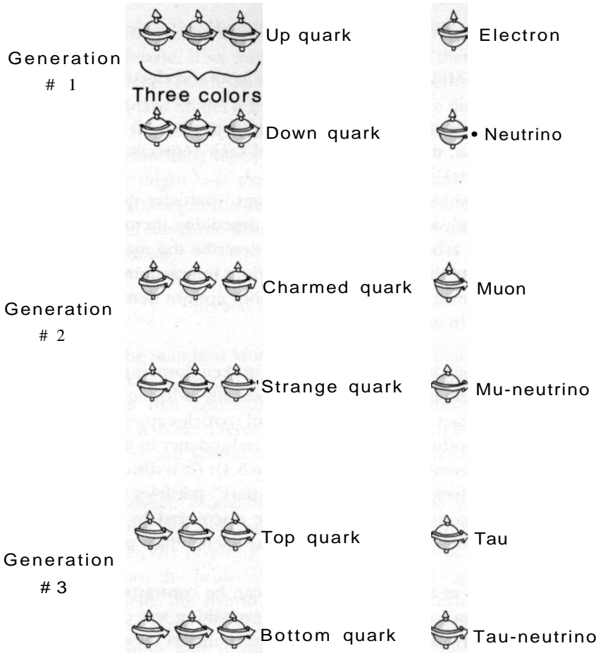
Figure 5.4. In the Standard Model, the first generation of particles consists of the "up" and "down" quark (in three colors, with their associated antiparticles) and the electron and neutrino. The embarrassing feature of the Standard Model is that there are three generation of such particles, each generation being nearly an exact copy of the previous generation. It's hard to believe that nature would be so redundant as to create, at a fundamental level, three identical copies of particles.
