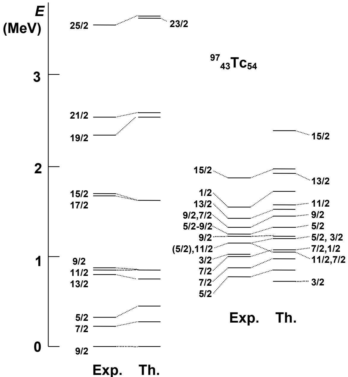
Figure 16.6. Comparison between the measured and the calculated spectrum with positive parity of {}^{97}\text{Tc} (von Brentano, 1981, p. 307). In the calculation, a proton with the states g_{9/2} and d_{5/2} has been coupled to {}^{96}\text{Mo} . This nucleus has been treated with the IBM1 by means of the parameters \varepsilon = 0.795 MeV, c_0' = -0.25 MeV, c_2' = -0.085 MeV, c_4' = 0.047 MeV, v_2 = 0.113 MeV and v_0 = 0 MeV (7.31). The fermion-boson term V_{BF} (16.18) has been calculated with expressions, which correspond largely to the equations (16.19) and (16.27).
