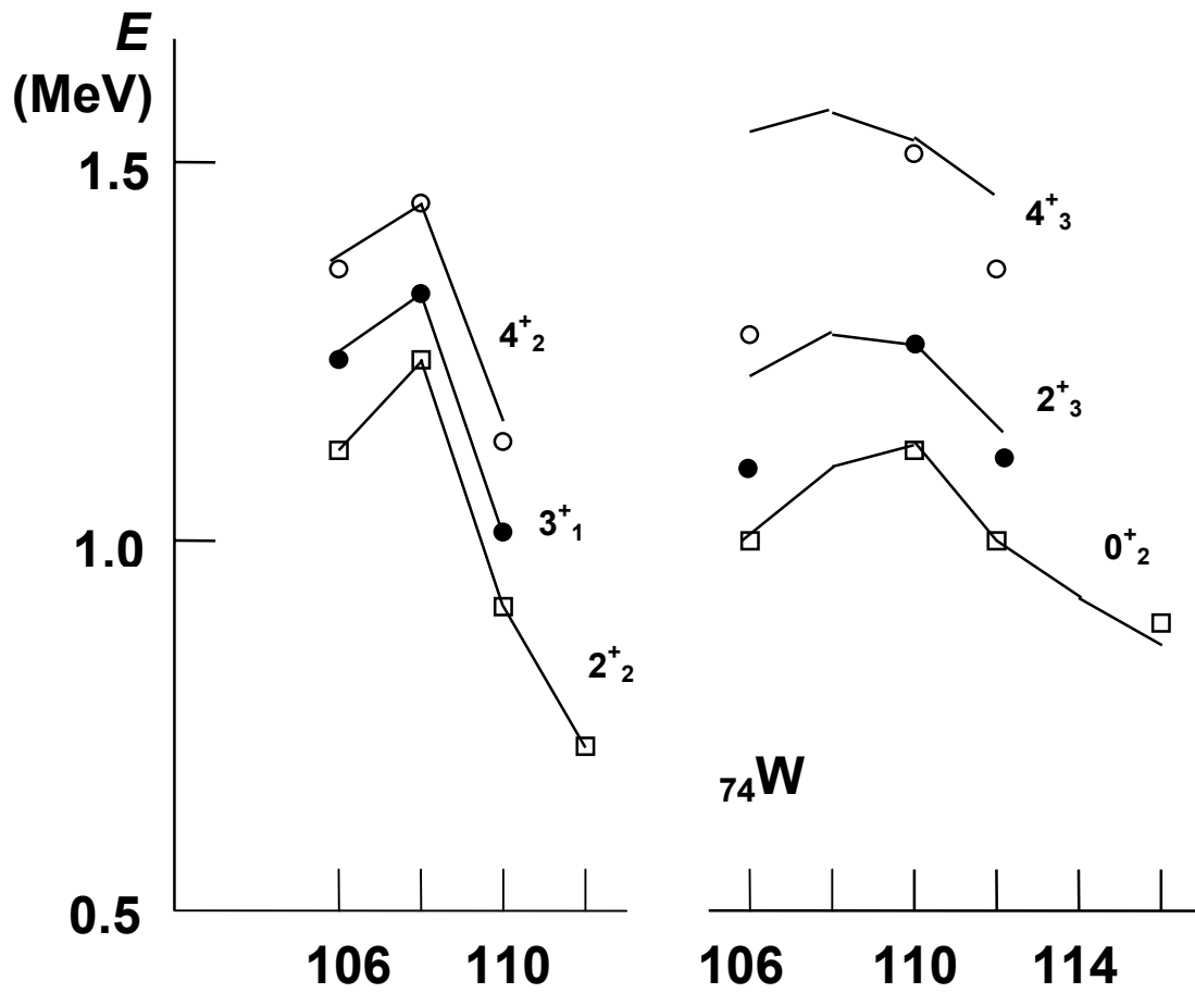
Figure 15.8. Comparison between measured and calculated energies of 6 levels of {}_{74}\text{W} with even numbers of neutrons 106 up to 116. The IBM2-Hamiltonian has been employed (Duval and Barrett, 1981, p. 494).
