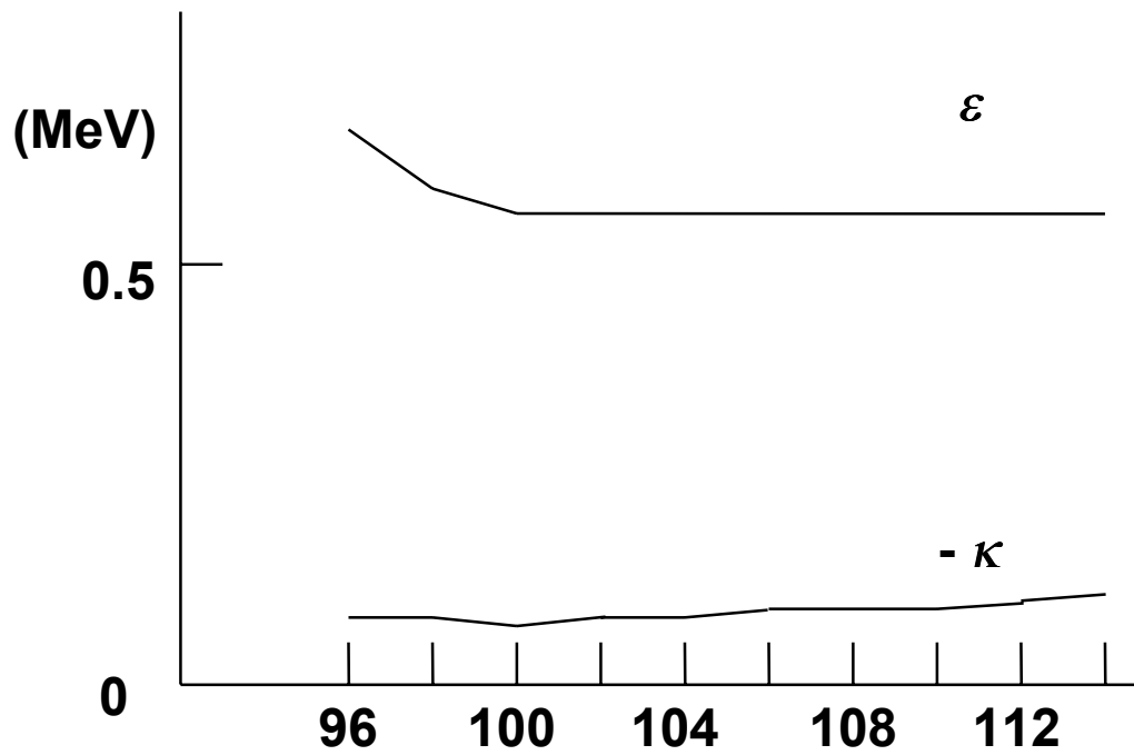
Figure 15.9. The parameters \kappa ( with negative values ) and \varepsilon employed for the IBM2-calculations shown in figures 15.7 and 15.8 for tungsten isotopes with even neutron numbers 96 up to 114 (Duval and Barrett, 1981, p. 495).
