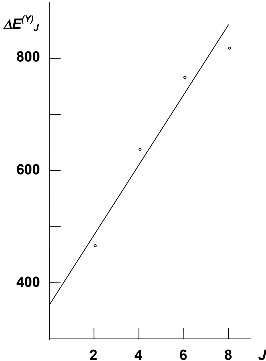
Figure 10.2. Energy differences \Delta E^{(Y)}_J = E^{(Y)}_J - E^{(Y)}_{J-2} between levels of the Y-series following each other of the nucleus ^{102}_{44}\text{Ru}_{58} according to figure 10.1. The straight line fitted in by eye yields the values c_4 = 125 keV and \varepsilon = 485 keV for the coefficients in (10.21).
