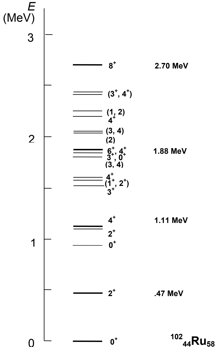
Figure 10.1. Measured spectrum of ^{102}\text{Ru} . The energies of the Y-series are given (Arima and Iachello, 1976a, p. 273).
