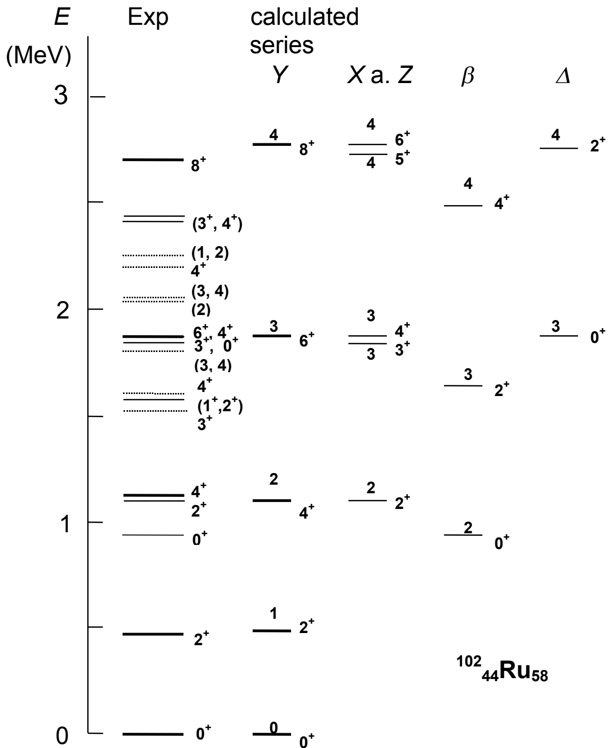
Figure 10.3. Comparison between the measured and the theoretical spectrum of 102 Ru. The spectrum is calculated by means of (10.19) and (10.18) with the parameters \varepsilon = 481 keV, c_0 = -18 keV, c_2 = 141 keV, c_4 = 144 keV and u_2 = 0 (Arima and Iachello, 1976a, p. 273). The numbers above or below the lines indicate the numbers of d -bosons.
