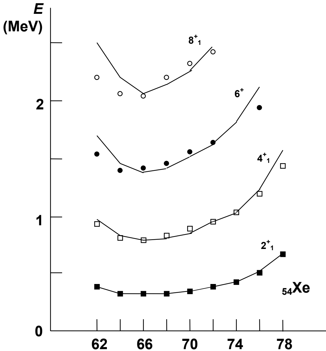
Figure 15.1. Comparison between the measured and the calculated energies of the levels 2^+_1 , 4^+_1 , 6^+_1 and 8^+_1 of isotopes of ^{54}\text{Xe} with even numbers of neutrons 62 up to 78. The IBM2-Hamiltonian has been employed (Scholten, 1980, p. 55).
