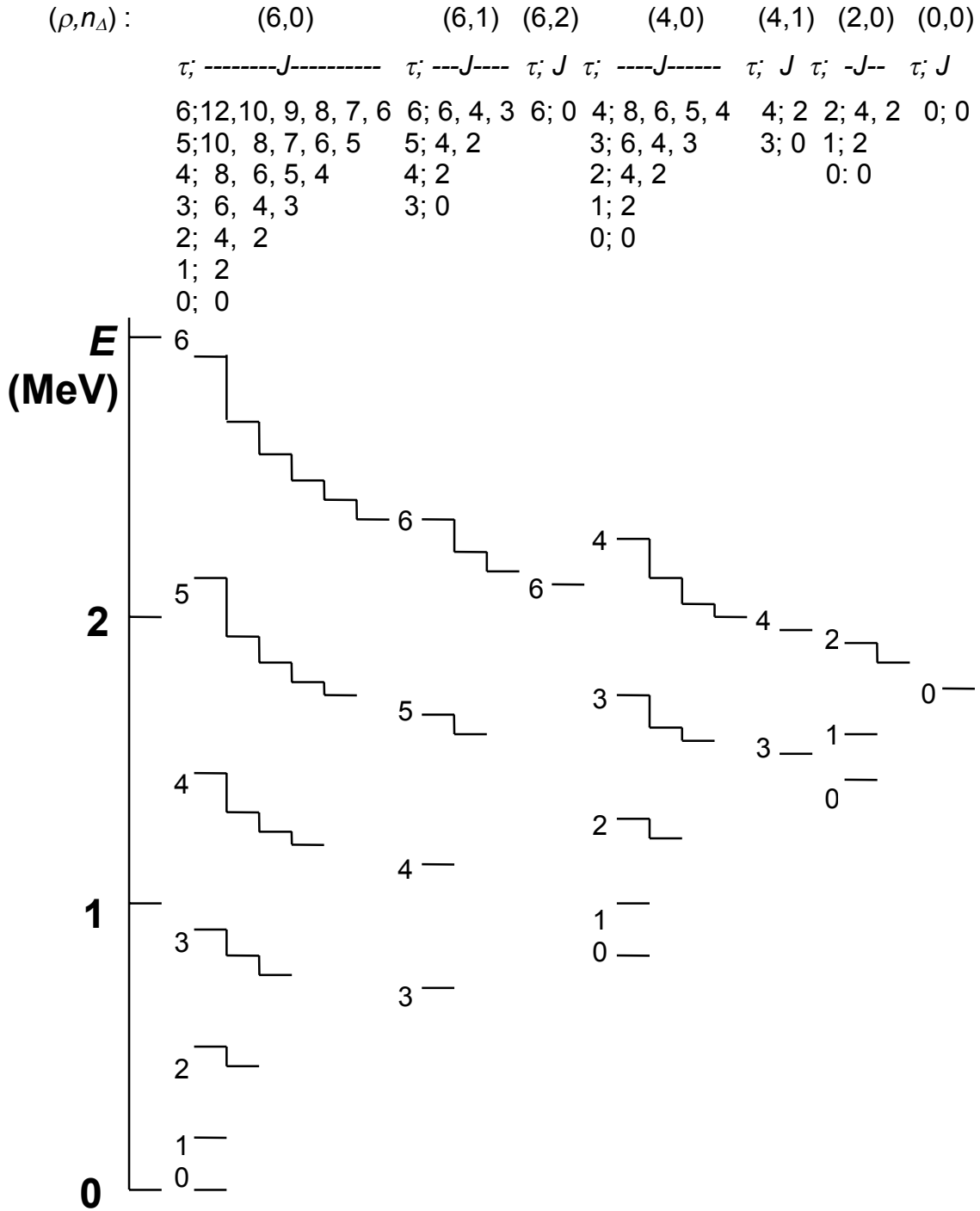
Figure 14.5. Typical spectrum of the so(6) limit. It is calculated by means of equation (14.61) and the values N = 6 , v_r = -30 keV, v_t = 40 keV and v_j = 5, 1 keV. The parameters \rho and \tau follow the rules (14.56) and (14.57). The values of n_\Delta and J are given by (14.58). All levels have positive parity. Level groups with the same \tau are joined together and labelled with the value of \tau . The J -values can be taken from the columns on top of the figure.
