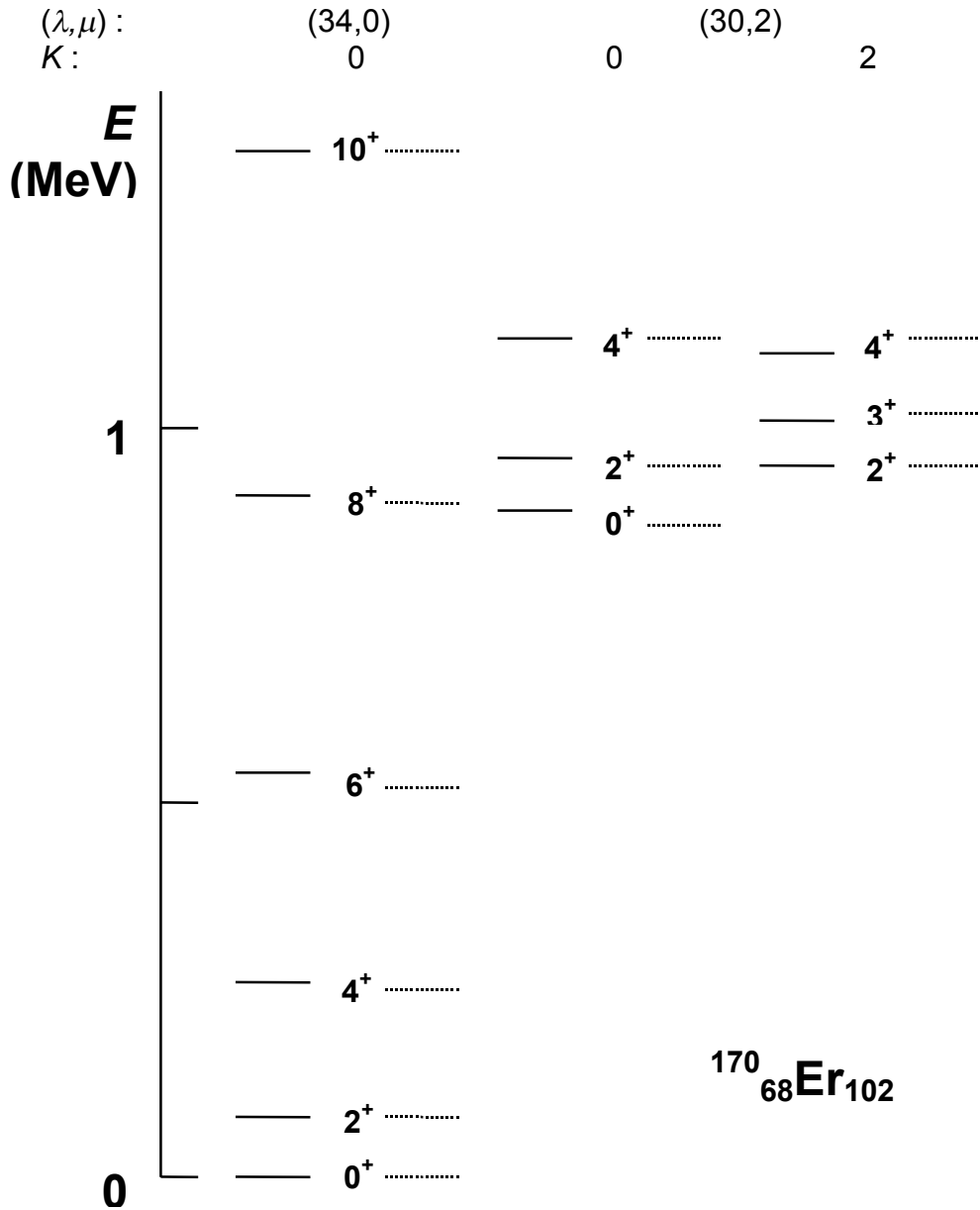
Figure 14.4. Comparison between the measured and the calculated su(3) -spectrum of ^{170}\text{Er} (Arima and Iachello, 1978, p. 215). The parameters N = 17 , v_j = 9.19 keV and v_q = -8.8 keV have been used with formula (14.52). Broken lines represent the calculated energies.
