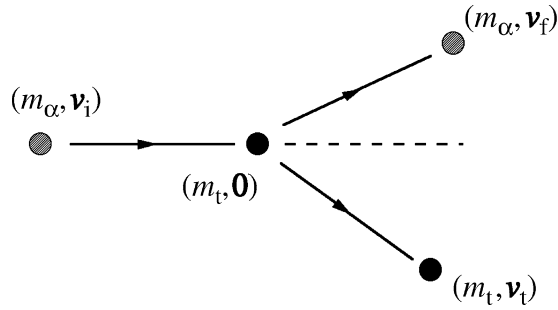
Figure C.1 Kinematics of the Geiger and Marsden experiment
