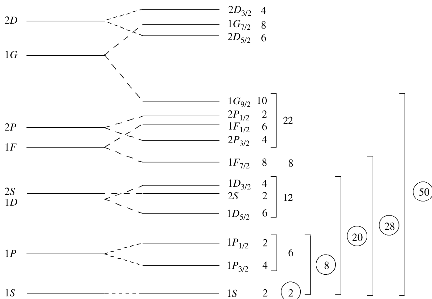
Figure 7.4 Low-lying energy levels in a single-particle shell model using a Woods--Saxon potential plus spin--orbit term; circled integers correspond to nuclear magic numbers
