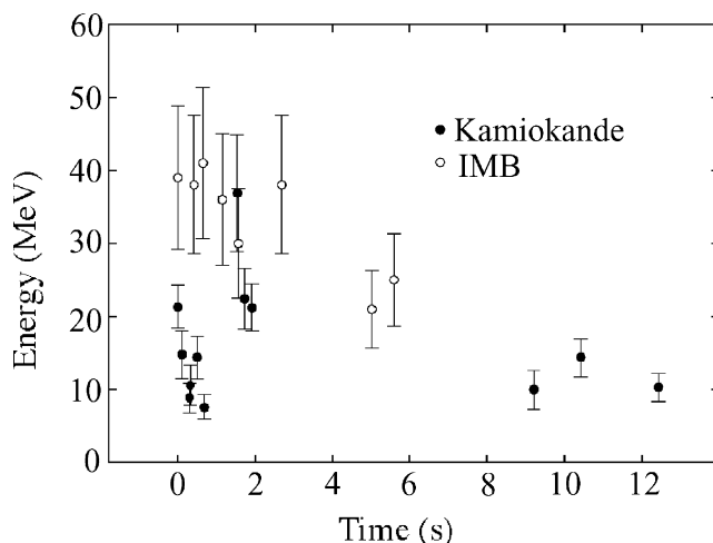
Figure 9.7 Data for neutrinos from SN1987A detected in the Kamiokande and IMB experiments: the threshold for detecting neutrinos in the experiments are 6 MeV (Kamiokande) and 20 MeV (IMB) -- in each case the first neutrino detected is assigned the time zero
