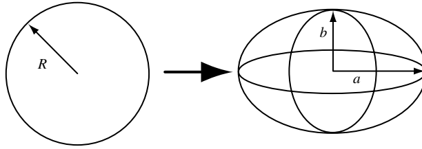
Figure 2.14 Deformation of a heavy nucleus
