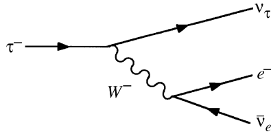
Figure 3.2 Dominant Feynman diagram for the decay \tau^- \rightarrow e^- \bar{\nu}_e \nu_\tau
