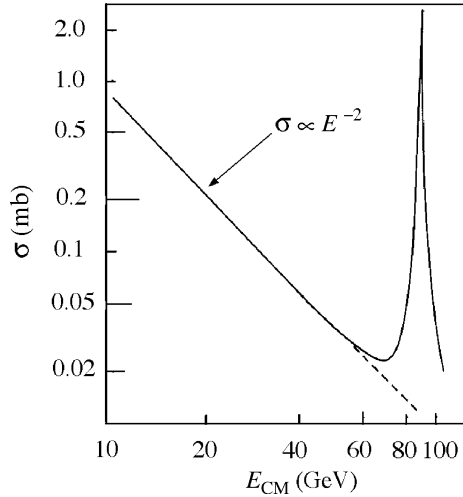
Figure 6.20 Total cross-section for the reaction e^+e^- \rightarrow \mu^+\mu^-
