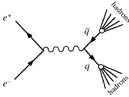
Figure 3.8 Production mechanism for the reaction e^+e^- \rightarrow q\bar{q}
