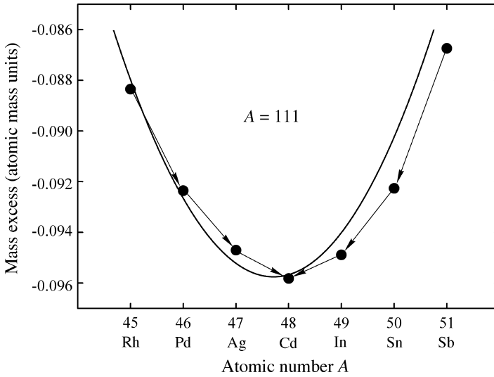
Figure 2.12 Mass parabola of the A = 111 isobars: the circles are experimental data and the curve is the prediction of the SEMF -- possible \beta -decays are indicated by arrows
