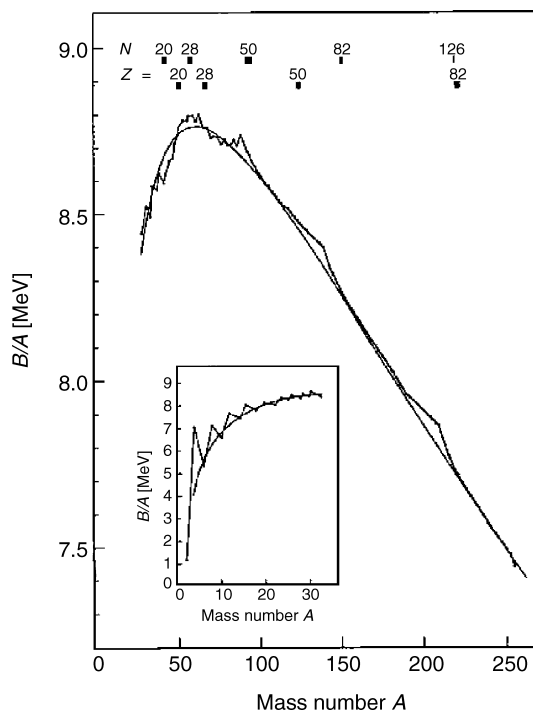
Figure 7.3 Binding energy per nucleon for even values of A : the solid curve is the SEMF (from Bo69)
