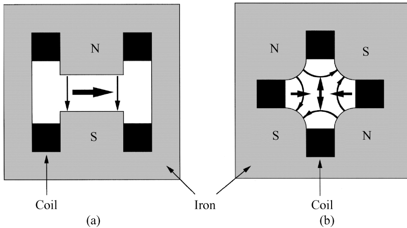
Figure 4.4 Cross-section of (a) a typical bending (dipole) magnet, and (b) a focusing (quadrupole) magnet; the thin arrows indicate field directions; the thick arrows indicate the force on a negative particle travelling into the paper
