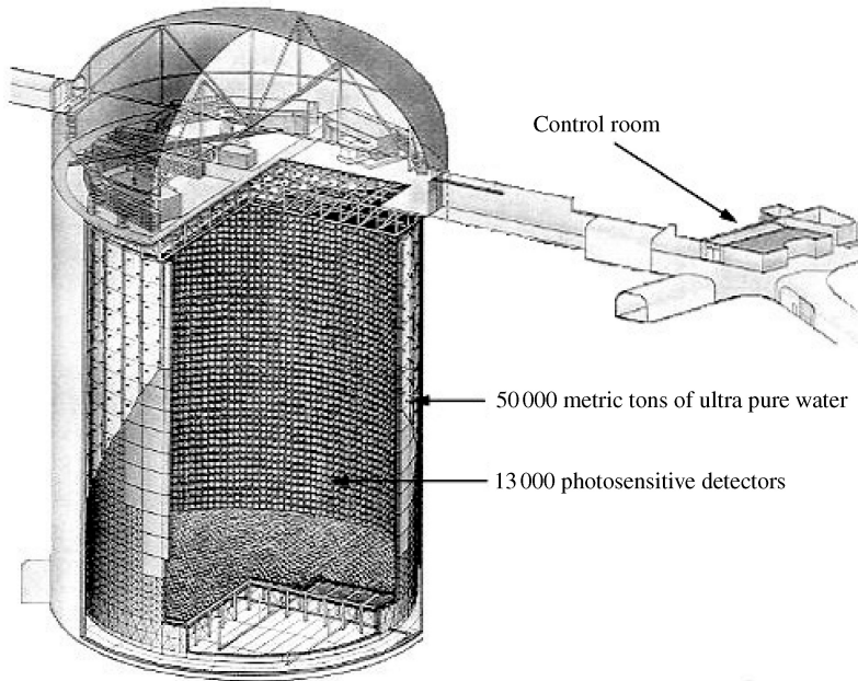
Figure 3.3 A schematic diagram of the Super Kamiokande detector (adapted from an original University of Hawaii, Manoa, illustration -- with permission)
