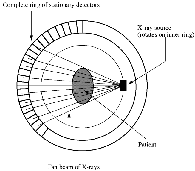
Figure 8.12 Schematic diagram of the arrangement for a CT X-ray scanner
