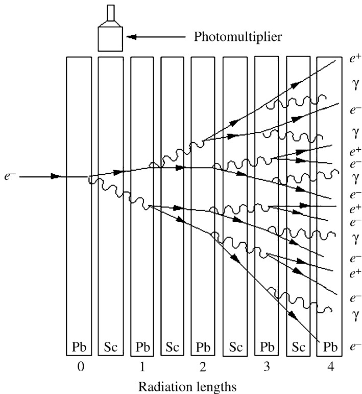
Figure 4.17 Approximate development of an electromagnetic shower in a sampling calorimeter assuming the simple model described in the text; the calorimeter consists of alternate layers of lead (Pb) and a scintillator (Sc), the latter attached to photomultipliers (one only shown)
