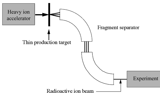
Figure 9.10 An energetic particle (typically several tens of MeV/u to GeV/u) is fragmented in a nuclear reaction in a thin target, and radioactive reaction products are separated in-flight and transported as a secondary beam to the experiment
