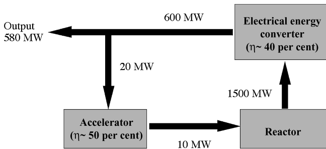
Figure 9.15 Possible energy flows in an energy amplifier system; the conversion efficiencies are denoted by \eta
