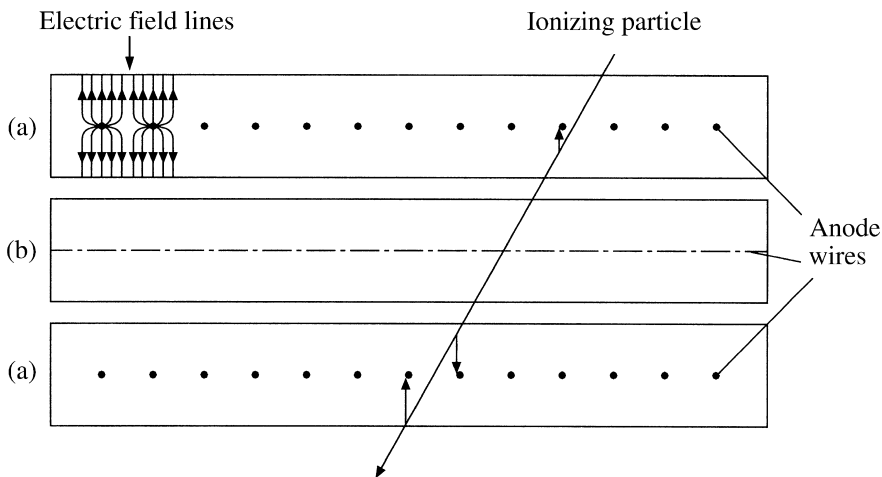
Figure 4.13 A group of three planes of an MWPC (from Po00 with kind permission of Springer Science and Business Media)
