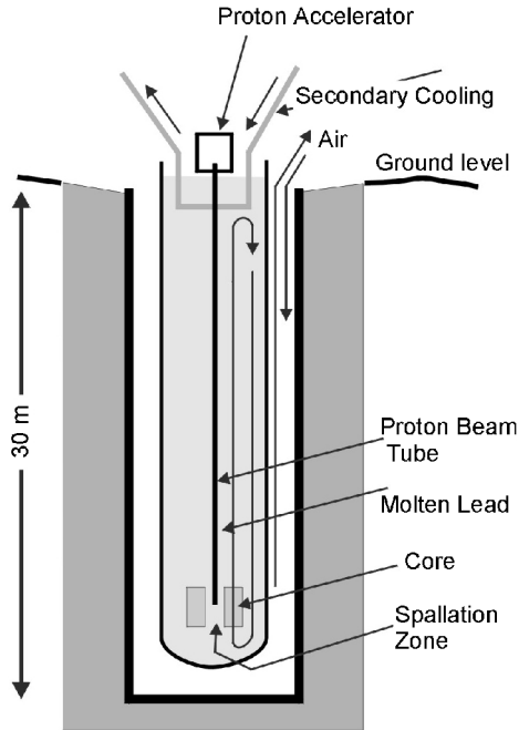
Figure 9.14 Schematic diagram of a possible configuration of an energy amplifier; in this design the coolant and spallation metal is molten lead (from Sc01, copyright Cavendish Press Ann Arbor 2001, with permission)
