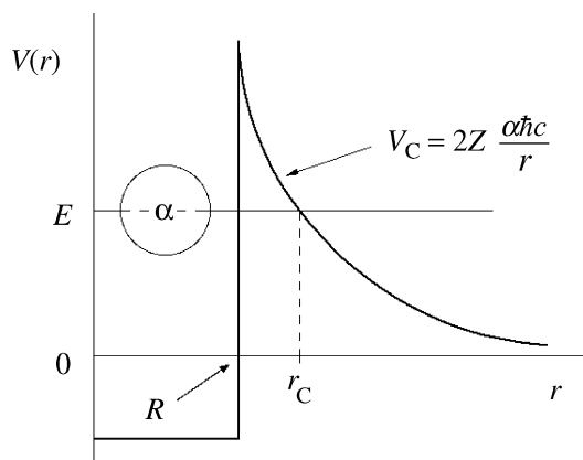
Figure 7.8 Schematic diagram of the potential energy of an \alpha -particle as a function of its distance r from the centre of the nucleus
