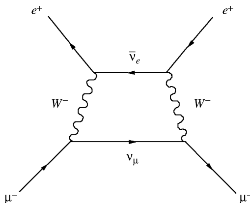
Figure 6.18 Higher order contribution to the reaction e^+\mu^- \rightarrow e^+\mu^- from the exchange of two W -bosons
