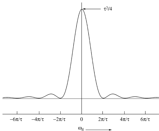
Figure A.2 The function \left[ \frac{\sin^2(\frac{1}{2}\omega_{fi}t)}{\omega_{fi}^2} \right]
