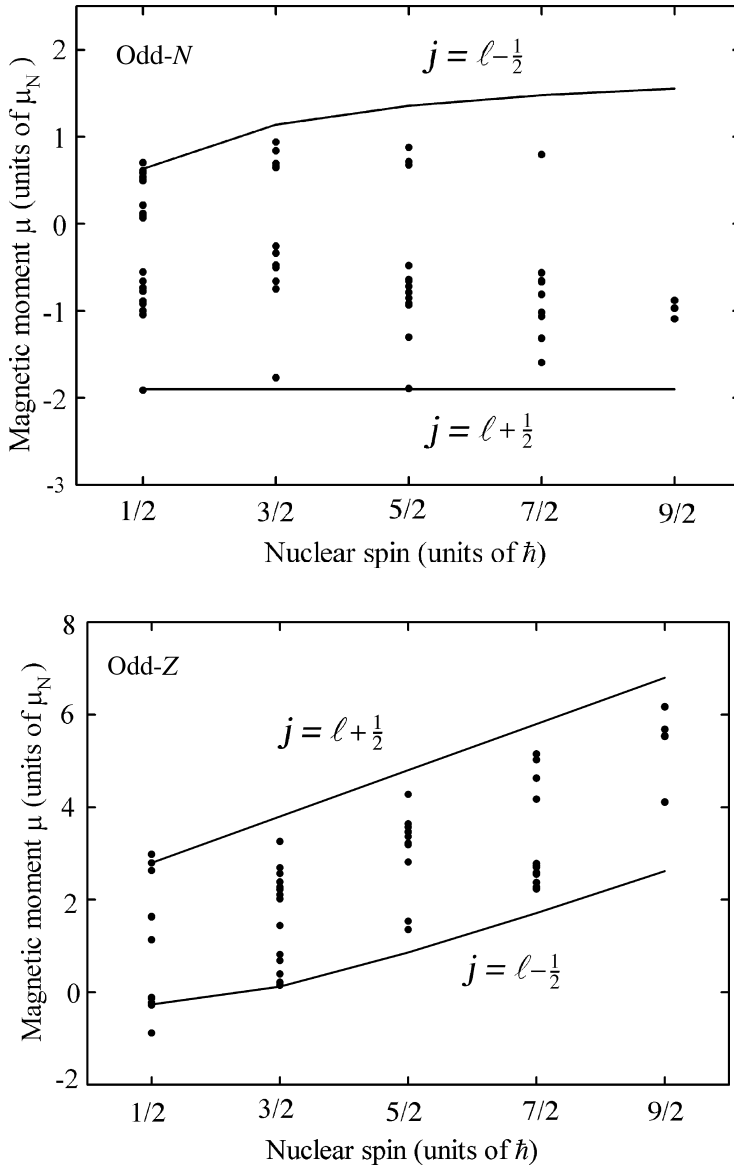
Figure 7.5 Magnetic moments for odd- N , even- Z nuclei (upper diagram) and odd- Z , even- N (lower diagram) as functions of nuclear spin compared with the predictions of the single-particle shell model (the Schmidt lines)
