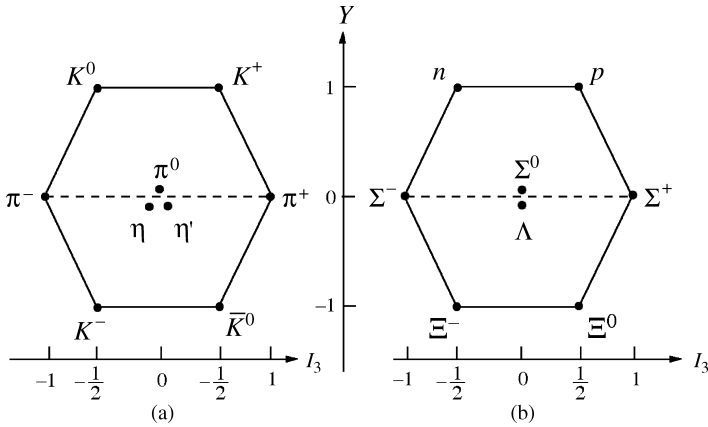
Figure 3.11 The lowest-lying states with (a) J^P = 0^- and (b) J = \frac{1}{2}^+ that are composed of u , d and s quarks
