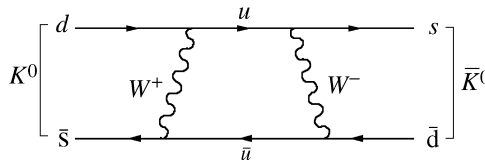
Figure 6.16 Example of a process that can convert a K^0 state to a \bar{K}^0 state
