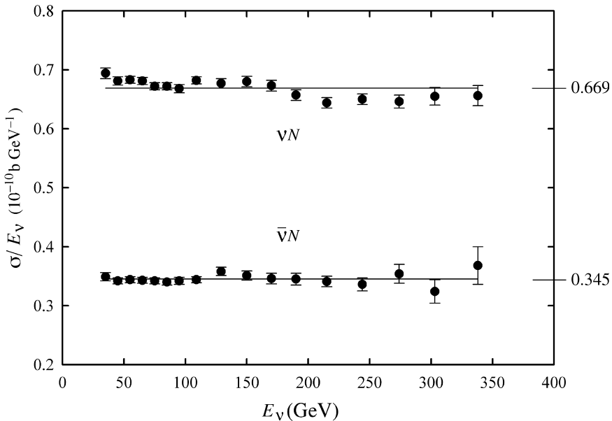
Figure 6.15 Neutrino and antineutrino total cross-sections (data from Se97)
