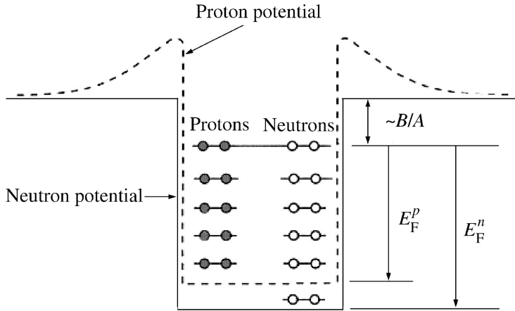
Figure 7.2 Proton and neutron potentials and states in the Fermi gas model
