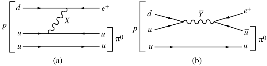
Figure 9.6 Examples of processes that contribute to the proton decay mode p \rightarrow \pi^0 + e^+
