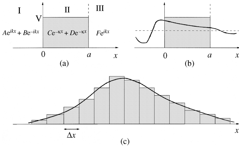
Figure A.1 Rectangular barrier with (a) wavefunction solutions, and (b) form of the incoming and outgoing waves; (c) modelling an arbitrary smooth barrier as a series of rectangular barriers
