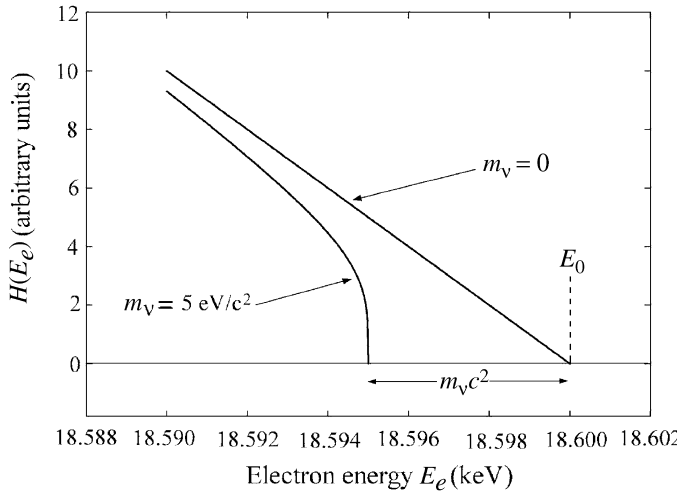
Figure 7.12 Expected Kurie plot for tritium decay very close to the end-point of the electron energy spectrum for two cases: m_\nu = 0 and m_\nu = 5 \text{ eV}/c^2
