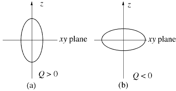
Figure 7.6 Shapes of nuclei leading to (a) Q > 0 (prolate), and (b) Q < 0 (oblate)
