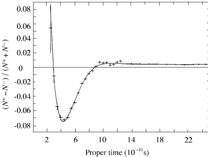
Figure 6.17 The charge asymmetry observed for K^0 \rightarrow \pi^- e^+ \nu_e and \bar{K}^0 \rightarrow \pi^+ e^- \bar{\nu}_e as a function of proper time, for a beam that is initially predominantly K^0 (adapted from Gj74, copyright Elsevier, with permission)
