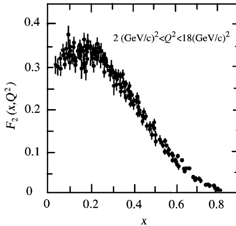
Figure 5.14 The structure function F_2 of the proton as a function of x , for Q^2 between 2 and 18 (\text{GeV}/c)^2 (reproduced from At82 with kind permission of Springer Science and Business Media)
