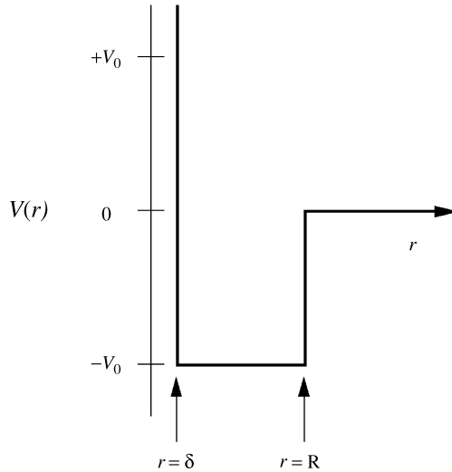
Figure 7.1 Idealized square well representation of the strong interaction nucleon--nucleon potential. The distance R is the range of the nuclear force and \delta \ll R is the distance at which the short-range repulsion becomes important. The depth V_0 is approximately 40 MeV
