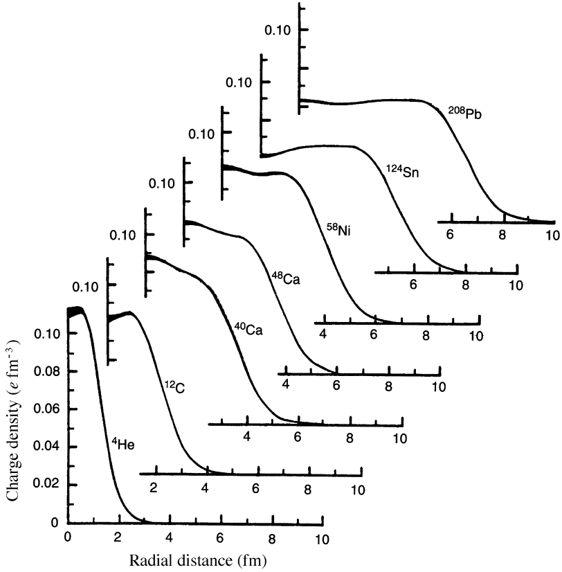
Figure 2.4 Radial charge distributions \rho_{\text{ch}} of various nuclei, in units of e \text{ fm}^{-3} ; the thickness of the curves near r = 0 is a measure of the uncertainty in \rho_{\text{ch}} (adapted from Fr83)
