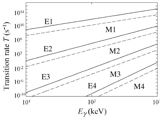
Figure 7.13 Transition rates using single-particle shell model formulas of Weisskopf as a function of photon energy for a nucleus of mass number A = 60
