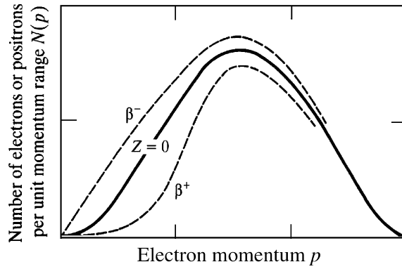
Figure 7.10 Predicted electron spectra: Z = 0 , without Fermi screening factor; \beta^\pm , with Fermi screening factor
