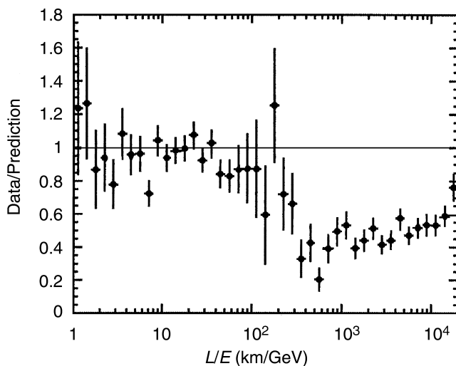
Figure 3.4 Data from the Super Kamiokande detector showing evidence for neutrino oscillations in atmospheric neutrinos (adapted from As04, copyright American Physical Society)
