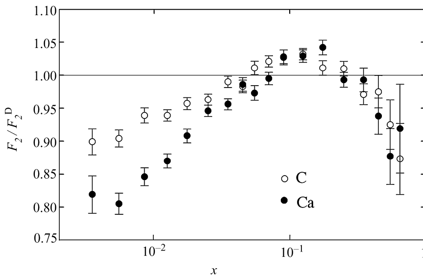
Figure 9.9 The ratios of the F_2 structure function found from nuclear targets to that found from deuterium, as a function of the scaling variable x (Carbon data from Ar95, calcium data from Am95)
