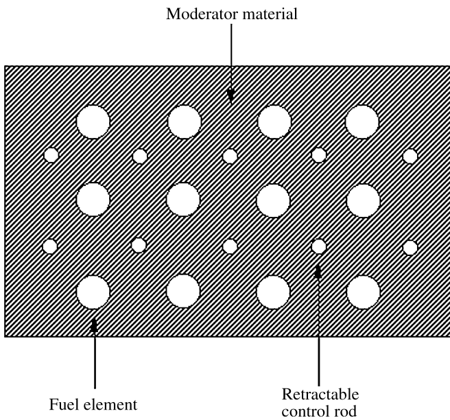
Figure 8.3 Sketch of the elements of the core of a reactor
