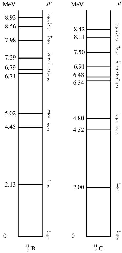
Figure 3.9 Low-lying energy levels with spin-parity J^P of the mirror nuclei ^{11}_5\text{B} and ^{11}_6\text{C} . (data from Aj90)
