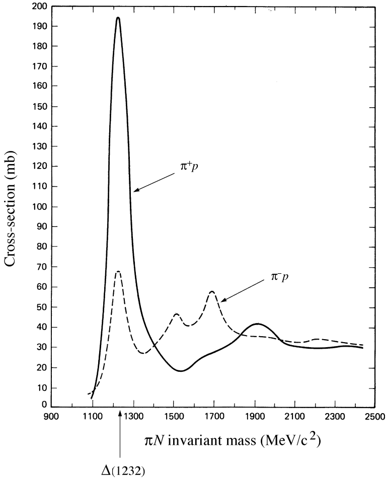
Figure 3.10 Total cross-sections for \pi^-p and \pi^+p scattering
