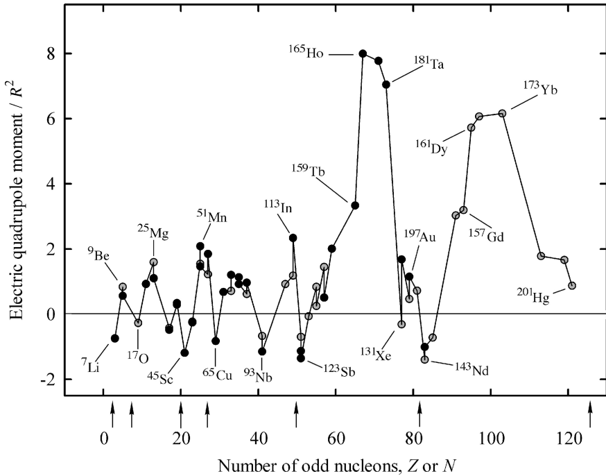
Figure 7.7 Some measured electric quadrupole moments for odd- A nuclei, normalized by dividing by R^2 , the squared nuclear radius: grey circles denote odd- N nuclei and black circles odd- Z nuclei; the solid lines have no theoretical significance and the arrows denote the position of closed shells
