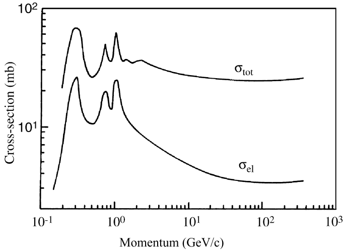
Figure 4.7 Total and elastic cross-sections for \pi^-p scattering as functions of the pion laboratory momentum
