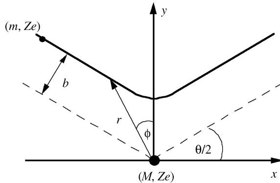
Figure C.2 Kinematics of Rutherford scattering
