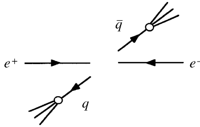
Figure 3.6 Mechanism for two-jet production in e^+e^- annihilation reaction
