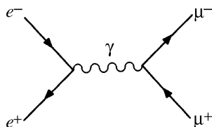
Figure 3.1 Single-photon exchange in the reaction e^+e^- \rightarrow \mu^+\mu^-
