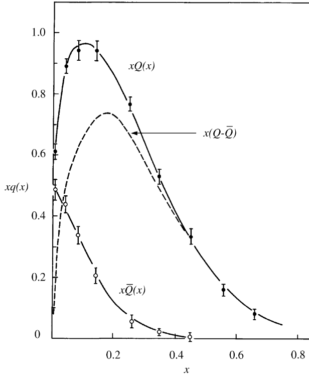
Figure 5.18 Quark and antiquark momentum distributions in the nucleon
