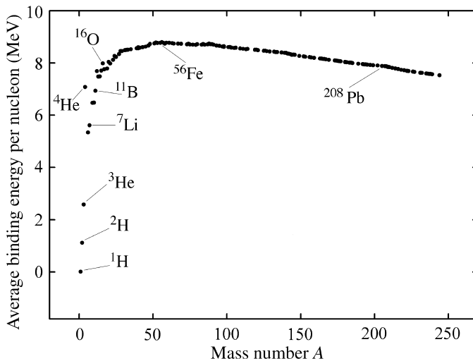
Figure 2.2 Binding energy per nucleon as a function of mass number A for stable and long-lived nuclei
