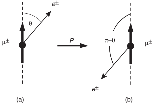
Figure 6.3 Effect of a parity transformation on muon decays: the thick arrows indicate the direction of the muon spin, while the thin arrows indicate the direction of the electron’s momentum
