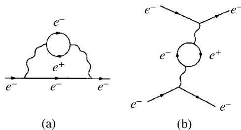
Figure 5.8 (a) A more complicated quantum fluctuation of the electron, and (b) the associated exchange process
