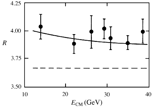
Figure 5.12 Measured values of the cross-section ratio R and the theoretical prediction from QCD for N_C = 3 colours; the dashed line shows the prediction without QCD corrections
