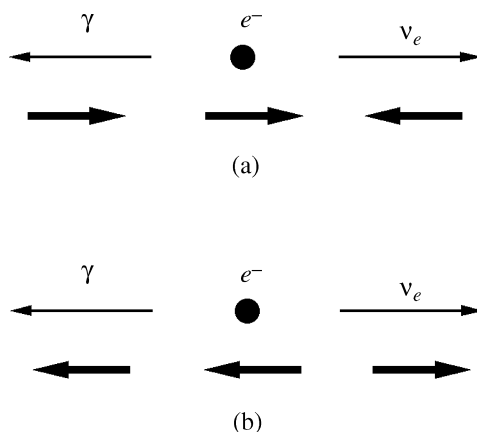
Figure 6.6 Possible helicities of the photon and neutrinos emitted in the reaction e^- + {}^{152}\text{Eu}(J=0) \rightarrow {}^{152}\text{Sm}(J=0) + \nu_e + \gamma for those events in which they are emitted in opposite directions. Experiment selects configuration (a)
