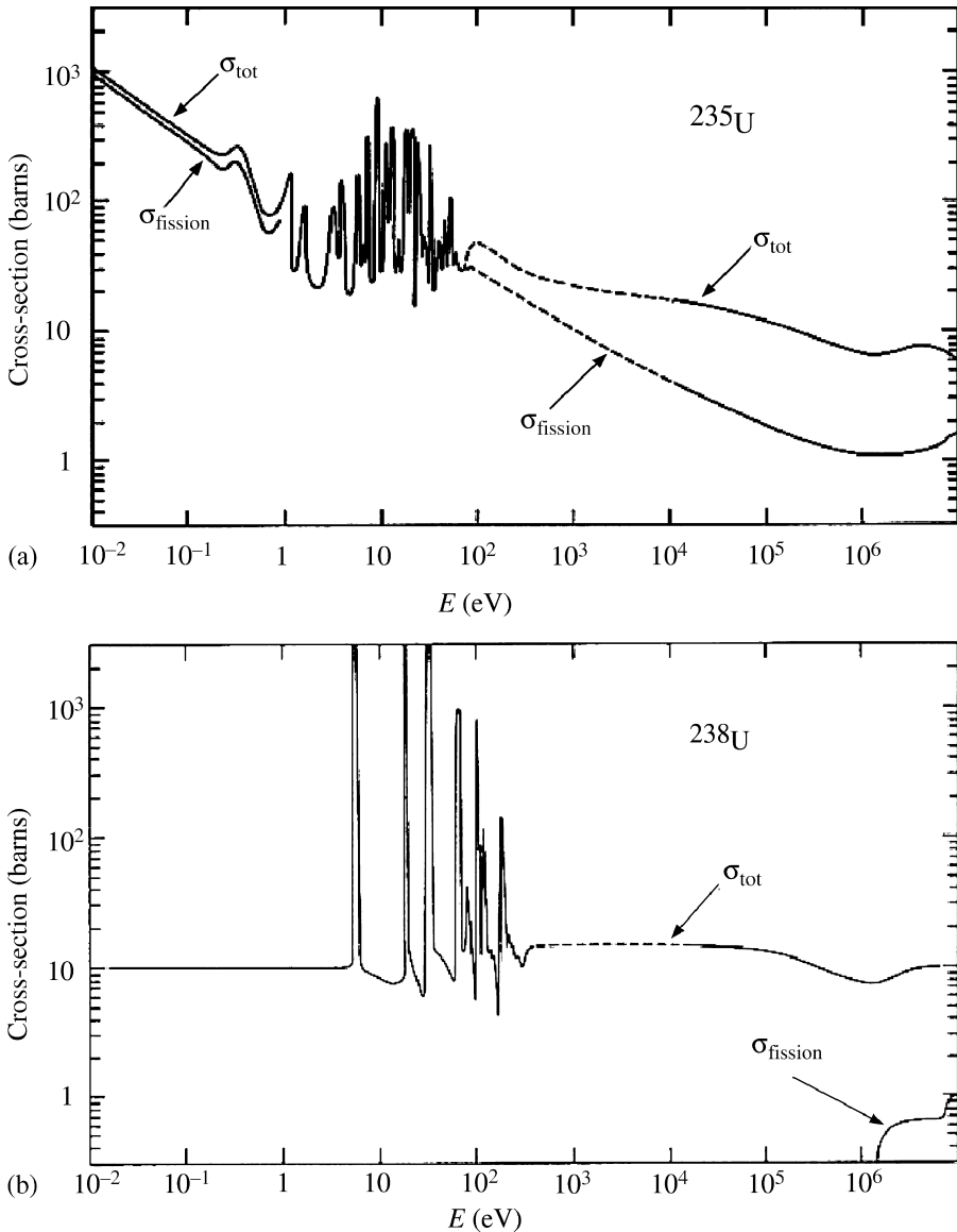
Figure 8.1 Total cross-section \sigma_{\text{tot}} and fission cross-section \sigma_{\text{fission}} as functions of energy for neutrons incident on (a) ^{235}\text{U} and (b) ^{238}\text{U} (adapted from Ga76, Courtesy of Brookhaven National Laboratory)
