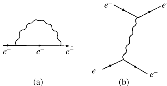
Figure 5.7 (a) The simplest quantum fluctuation of an electron, and (b) the associated exchange process
