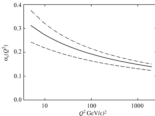
Figure 5.6 The running coupling constant \alpha_s corresponding to four flavours and a scale parameter \Lambda = 0.2 \pm 0.1 \text{ GeV}/c ; the dashed, solid and dot-dashed curves correspond to \Lambda = 0.1, 0.2 and 0.3 , respectively
