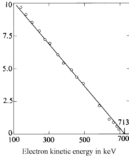
Figure 7.11 Kurie plot for the \beta -decay of ^{36}\text{Cl} (the y-axis is proportional to the function H(E_e) above)
