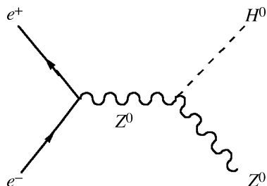
Figure 9.1 Dominant mechanism for Higgs boson production in e^+e^- annihilation
