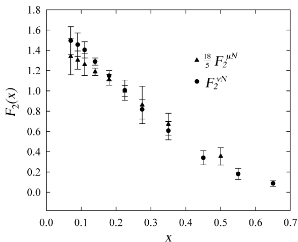
Figure 5.17 Comparison of F_2(x) from deep inelastic muon (data from Ar97) and neutrino (data from Se97) scattering experiments; the data points are the average over a range of Q^2 > 2 (\text{GeV}/c)^2 and the error bars express the range of data values within the Q^2 ranges
