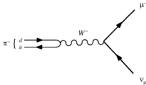
Figure 6.11 Quark diagram for the process \pi^- \rightarrow \mu^- + \bar{\nu}_\mu
