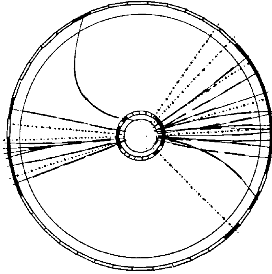
Figure 3.5 Two-jet event in e^+e^- collisions
