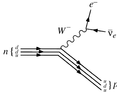
Figure 3.7 Spectator model quark Feynman diagram for the decay n \rightarrow pe^- \bar{\nu}_e
