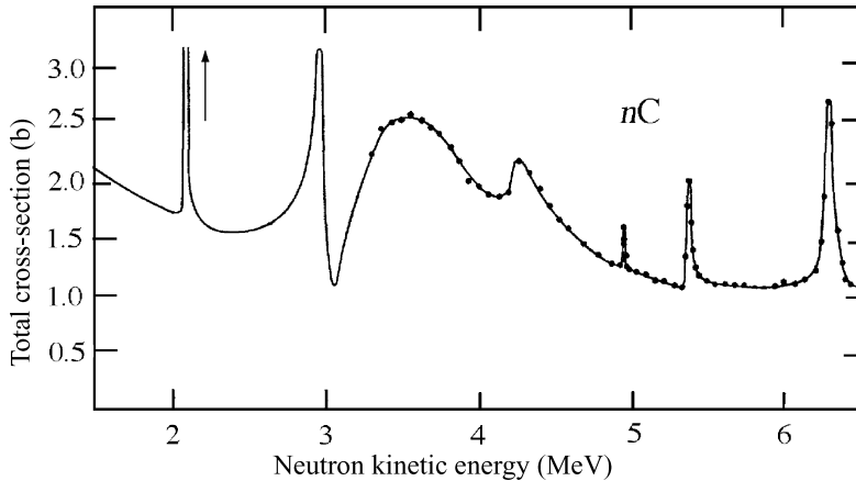
Figure 2.17 Total cross-section for n^{12}\text{C} interactions (adapted from Fo61. Copyright American Physical Society.)
