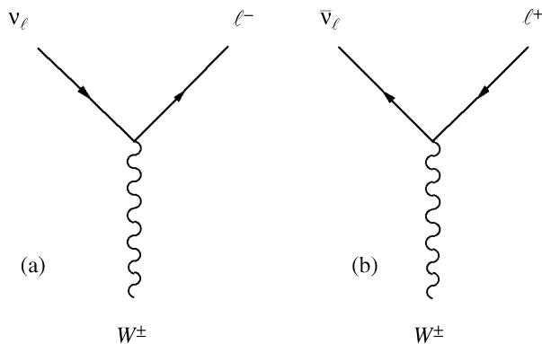
Figure 6.9 The two basic vertices for W^\pm -lepton interactions
