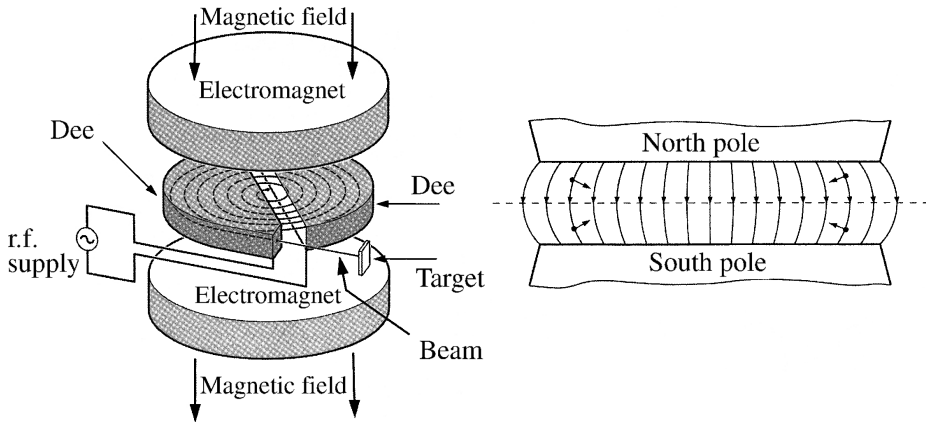
Figure 4.3 Schematic diagram of a cyclotron (adapted from Kr88, copyright John Wiley & Sons)
