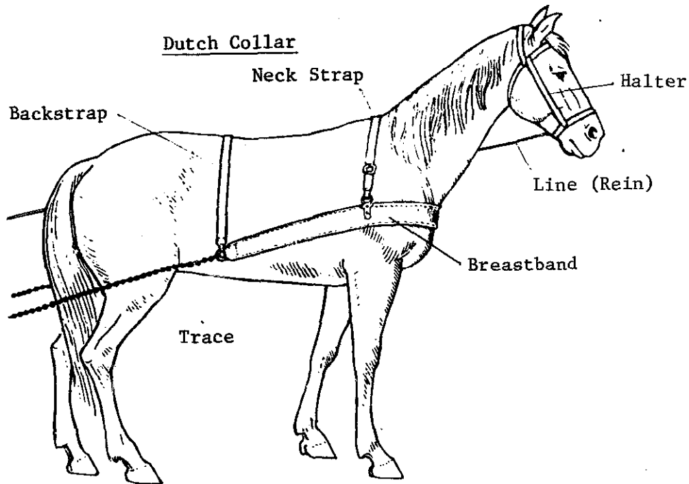
Breastband Harness, or Dutch Collar, Showing Correct Position of Straps
