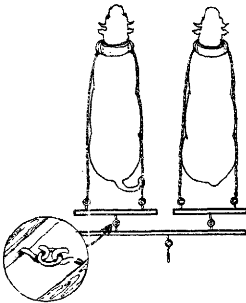
Doubletree to Implement Hitch (Standard)
