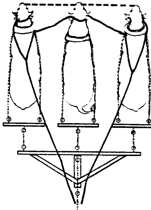
Three-Abreast Hitch
