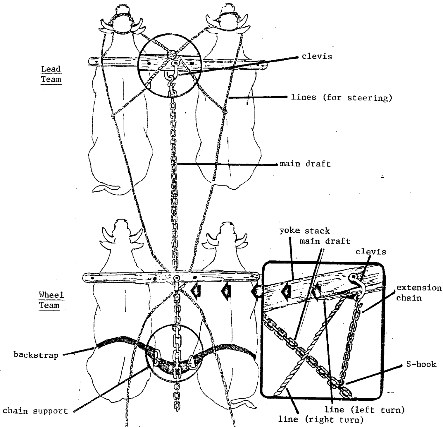
Tandem Yokes to Implement (with magnifications of hitchpoints)
