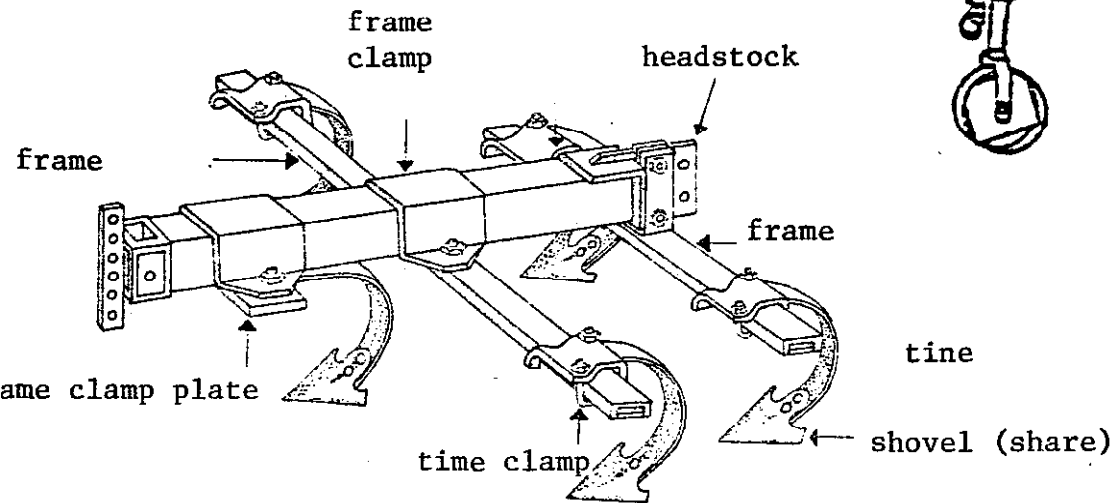
Five-Tooth Cultivator
