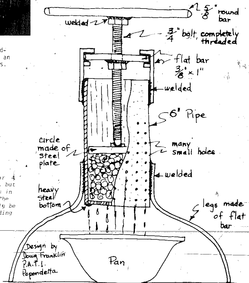
SIMPLE OIL PRESS (cutaway view)
