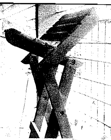
Stool made at Baitabag Vocational Centre, Madang, folds into a compact flat package. Joints are held with split rivets (made from nails) and washers.
