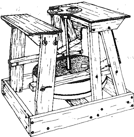
Another design: A simple kickwheel
