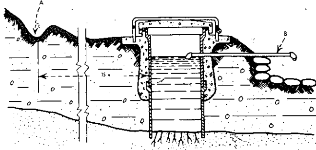
Fig. 34. PROPERLY PROTECTED SPRING (II)
