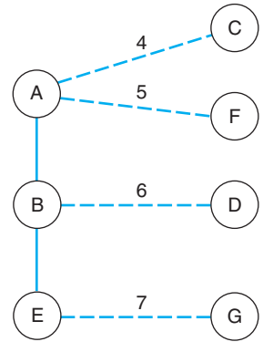
■ FIGURE 6.5D Third node added. Edge to node G updated.
