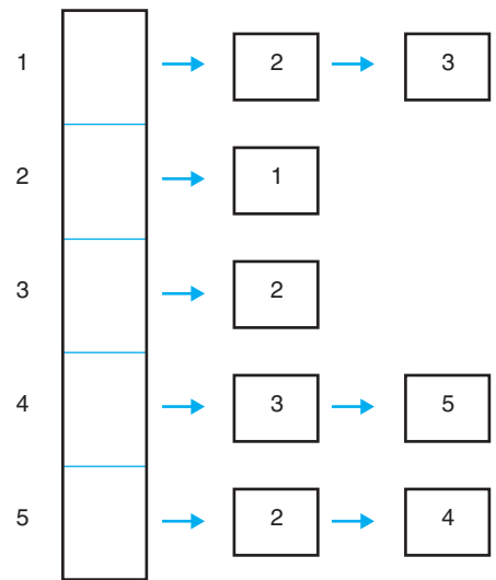
■ FIGURE 6.3B The adjacency list for the graph in Fig. 6.1(b)
