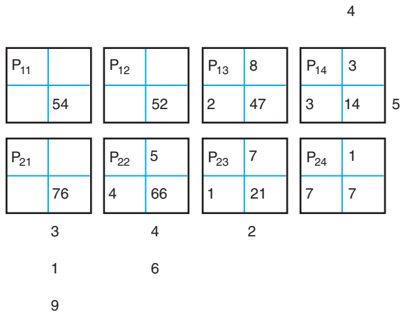
■ FIGURE 7.6F P_{12} and P_{21} are now done, P_{24} gets its first two numbers, and P_{13} , P_{22} , P_{14} , and P_{23} work on their next values
