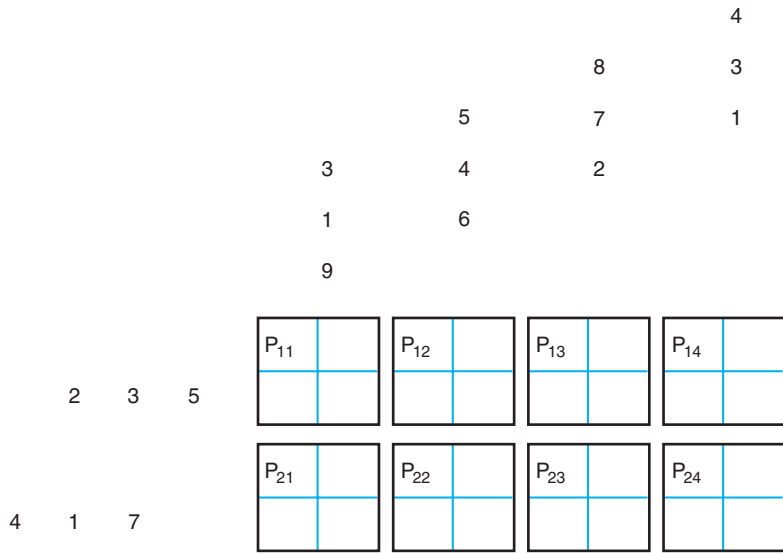
■ FIGURE 7.6A The initial mesh network setup
