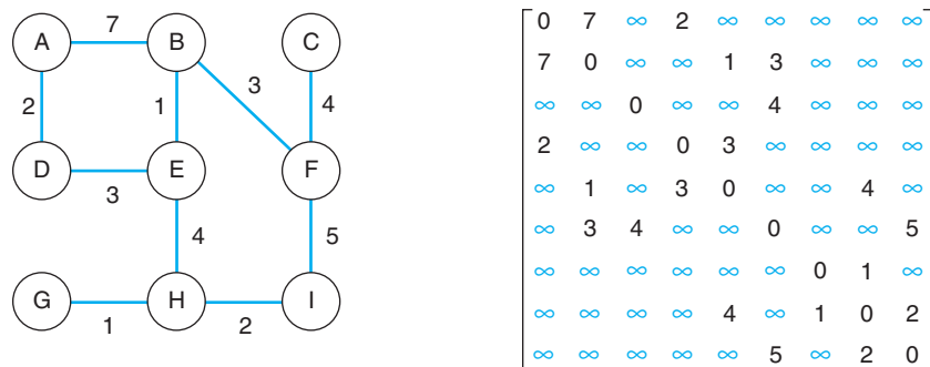
■ FIGURE 7.7 A weighted graph and its adjacency matrix
