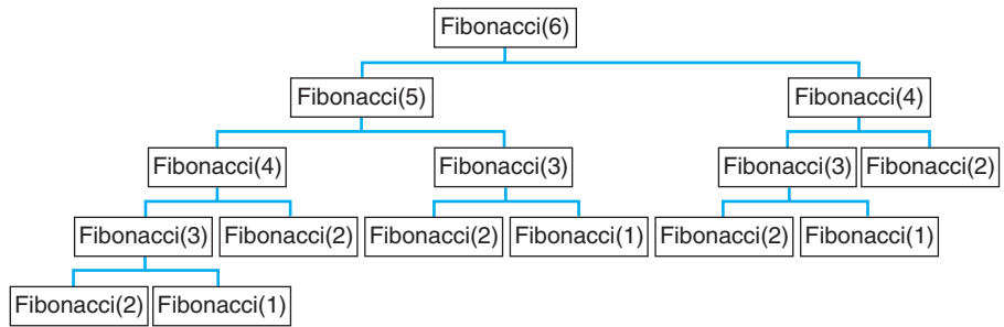
■ FIGURE 9.6 The calling sequence for Fibonacci(6)
