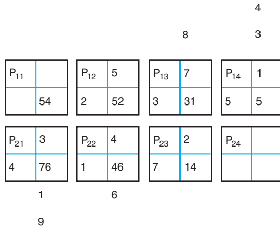
■ FIGURE 7.6E P_{11} is now finished and the result for row 1 column 1 is in its register; P_{12} , P_{21} , P_{13} , and P_{22} work on their next two values; and P_{14} and P_{23} get started
