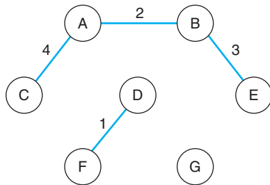
■ FIGURE 6.6E Fourth edge added
