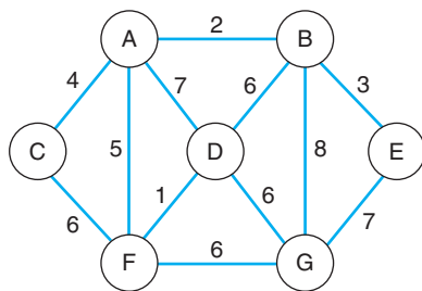
■ FIGURE 6.6A The original graph
