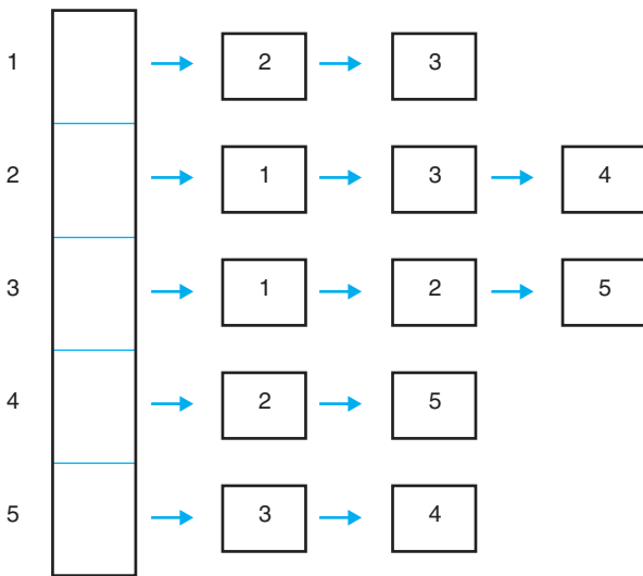
■ FIGURE 6.3A The adjacency list for the graph in Fig. 6.1(a)
