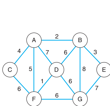
■ FIGURE 6.8A The original graph
