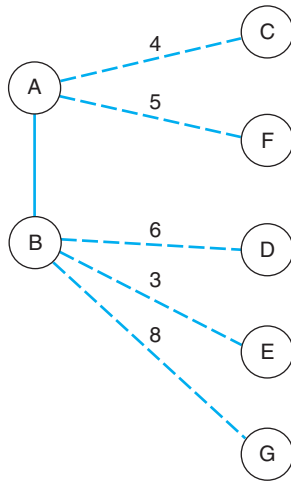
■ FIGURE 6.5C Second node added. Edges to nodes D, E, and G updated. (Solid lines show edges in the MST.)
