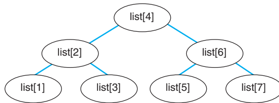
■ FIGURE 2.1 Decision tree for a search of a list of seven elements
