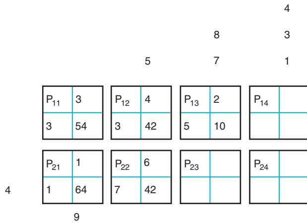
FIGURE 7.6D P_{11} , P_{12} , and P_{21} handle their next two numbers, and P_{13} and P_{22} join the process
