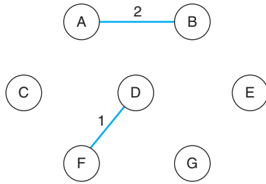
■ FIGURE 6.6C Second edge added
