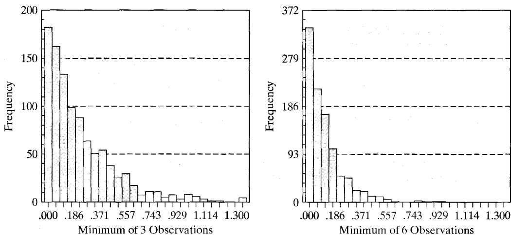
FIGURE C.4 Histograms of the Sample Minimum of 3 and 6 Observations.
