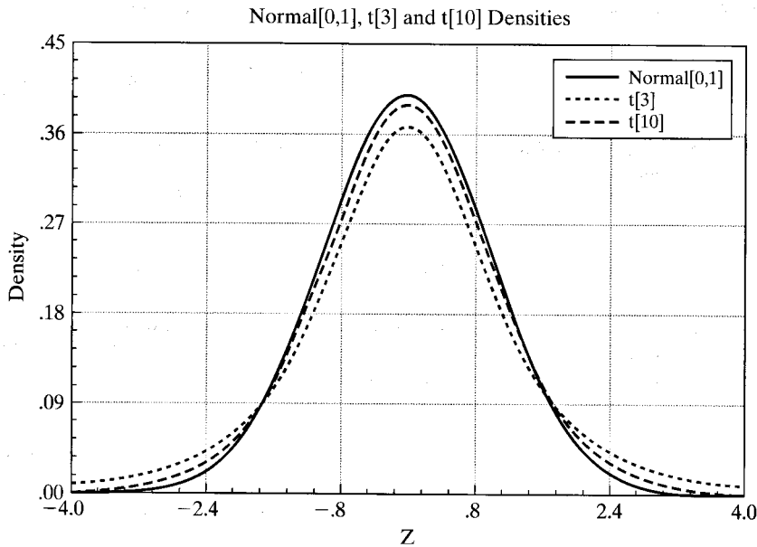
FIGURE B.3 The Standard Normal, t[3] and t[10] Distributions.
