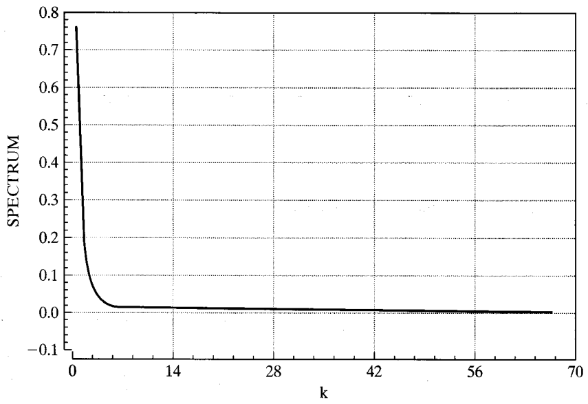
FIGURE 20.5 Spectrum for Real GNP.
