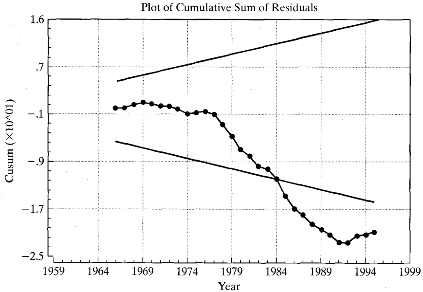
FIGURE 7.6 CUSUM Test.
