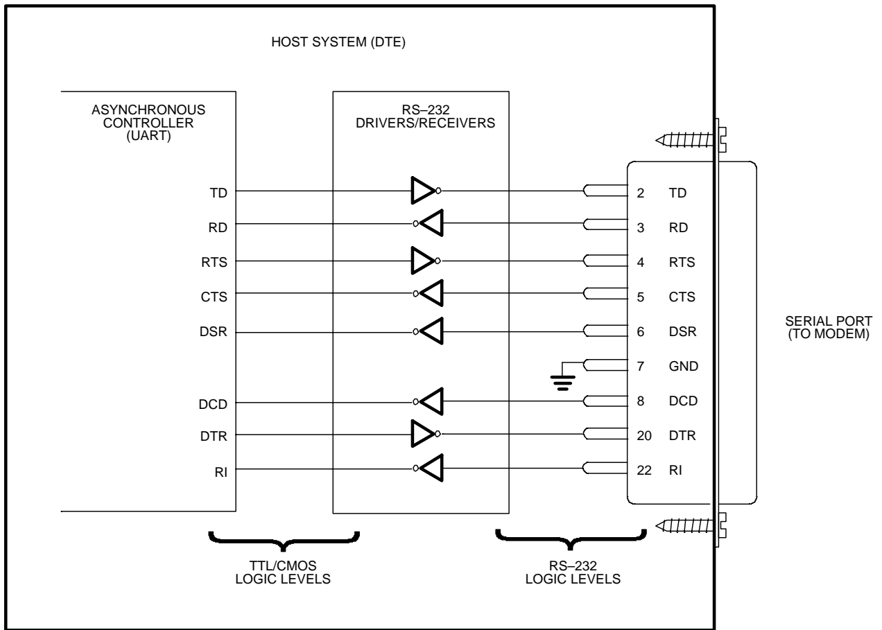
TYPICAL RS-232 MODEM APPLICATION Figure 3
