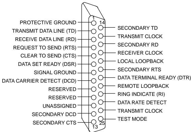
RS-232 CONNECTOR PIN ASSIGNMENTS Figure 2
