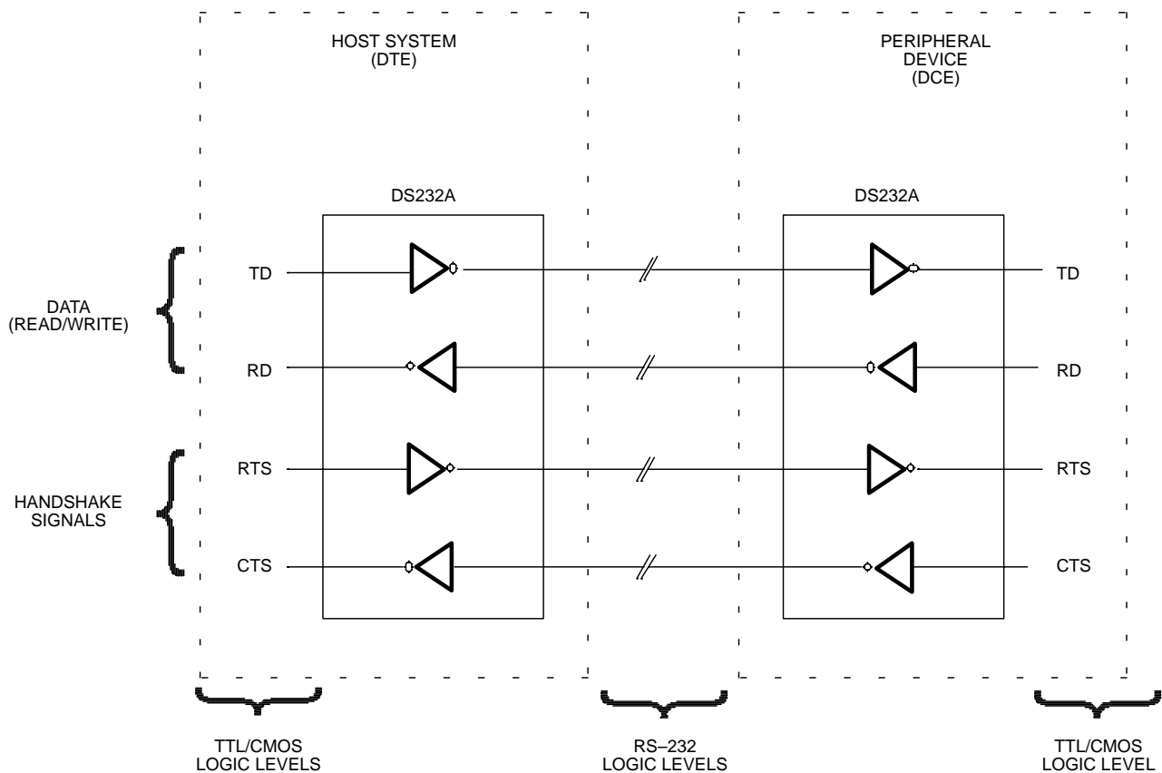
HALF-DUPLEX COMMUNICATION SCHEME Figure 5
