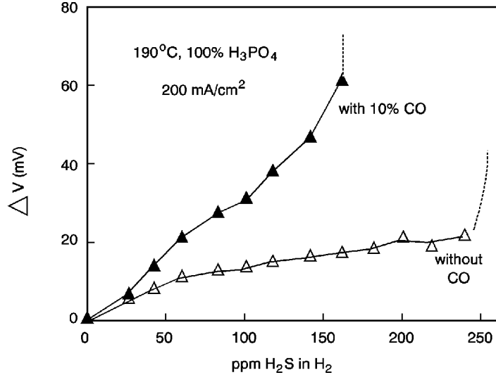
Figure 5-6 Effect of H 2 S Concentration: Ultra-High Surface Area Pt Catalyst (37)
