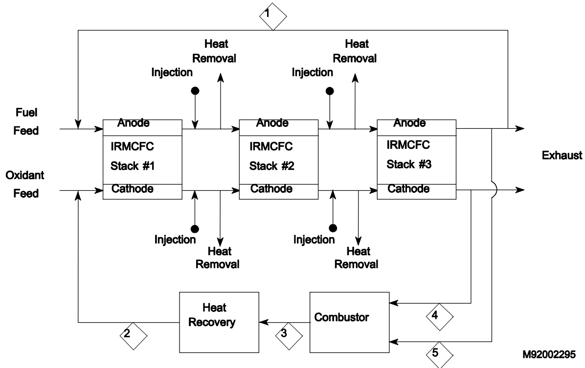
Figure 9-21 MCFC Network
