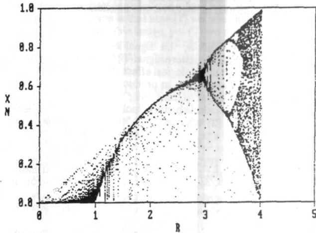
Figure 17. Chaos: The collected emergence of large-scale order from disorder. The apparent disorder actually contains hidden order.
