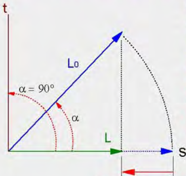
Lorentz-Fitzgerald Contraction
