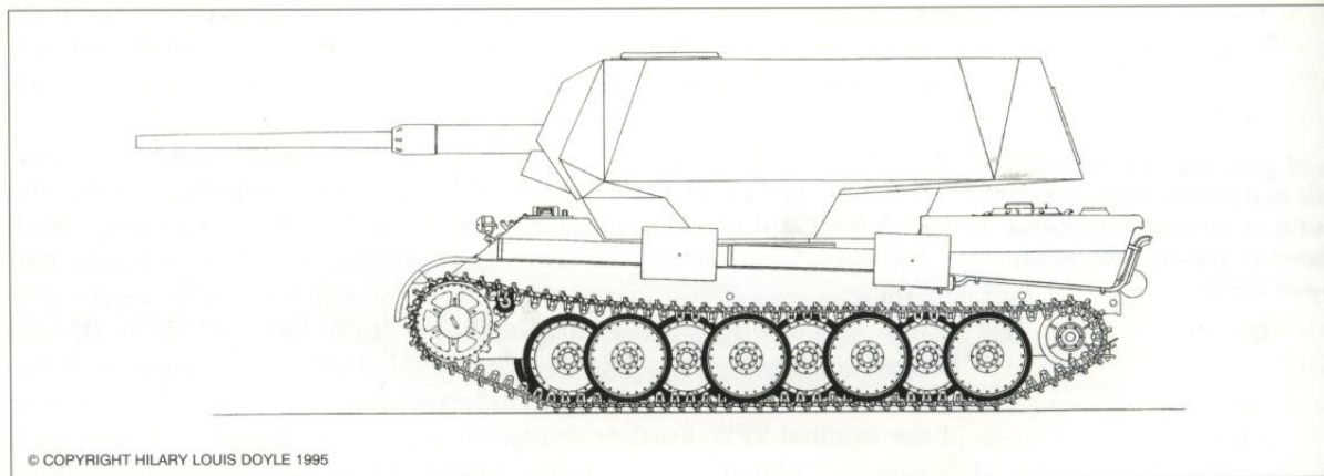
1:76 scale side view drawing of the Rheinmetall-Borsig proposal for '8.8 cm Flak 41 (Sf) mit Panther I Bauteilen' dated 24 October 1943. (Hilary Louis Doyle)
