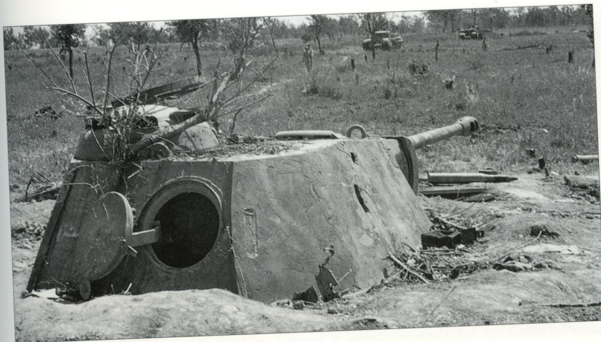
This Panther Ostwallturm was part of the Hitler line in Italy and was positioned near Monte Cassino. It consists of a normal Panther turret mounted on the Stahluntersatz (steel sub-base). Some of the Churchill tanks which it destroyed can be seen in the distance. (Imperial War Museum)
