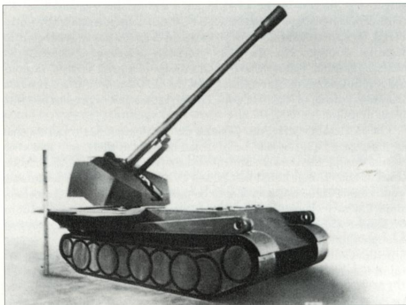
The Krupp model proposal for the 12.8 cm K. 43 (Sfl.) Kp. II, the Grille 12, with the firing platform folded down ready for firing.
