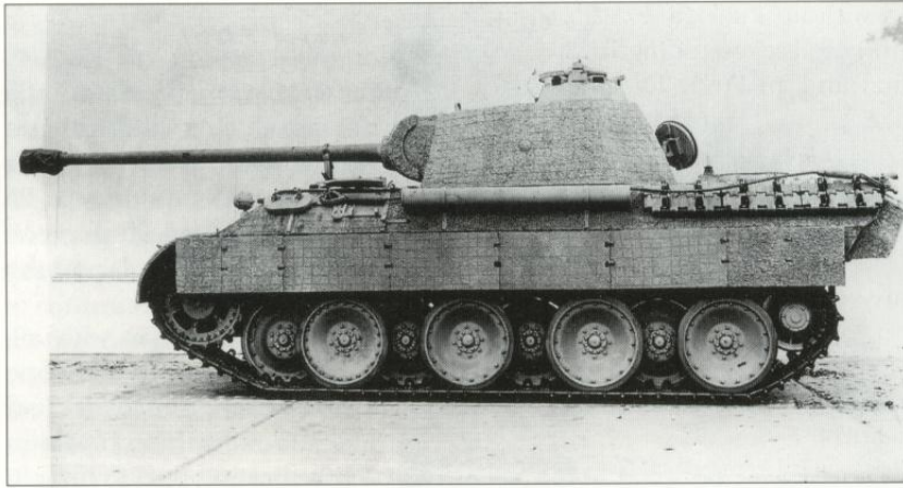
The Panther Ausf.A can be distinguished from the Ausf.D by the redesigned turret with the new commander's cupola. Note the pistol ports on the turret sides and the 'letter box' MG port in the hull were retained until late 1943.
