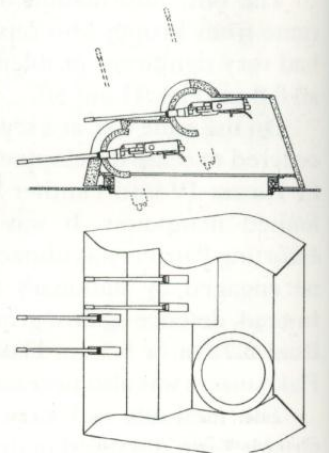
1:76 scale drawing of the Rheinmetall proposal for 'Turm Panther II mit Vierling MG151/20' dated 20 May 1943. (Hilary Louis Doyle)
