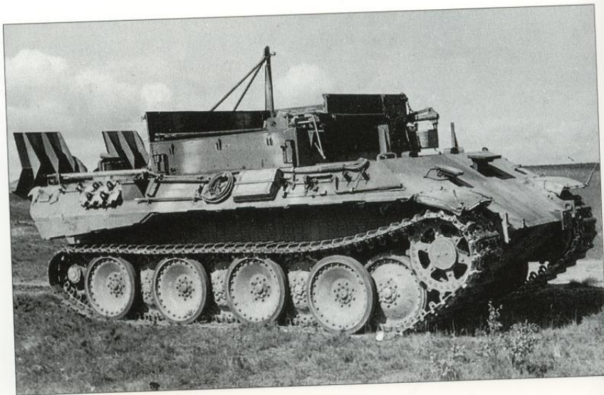
A Bergepanther based on the Panther Ausf.A (Fgst.Nr. 175644). This vehicle was captured and brought to England for examination. (Tank Museum)
