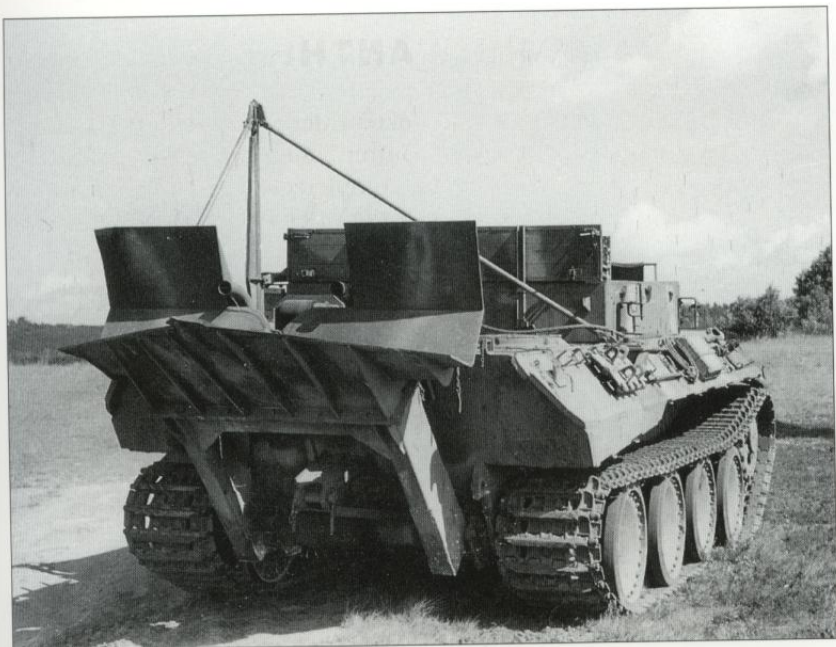
The rear view of the Bergepanther (Fgst.Nr. 175644). The spade was used to anchor the Bergepanther when the winch was retrieving vehicles. (Tank Museum)
