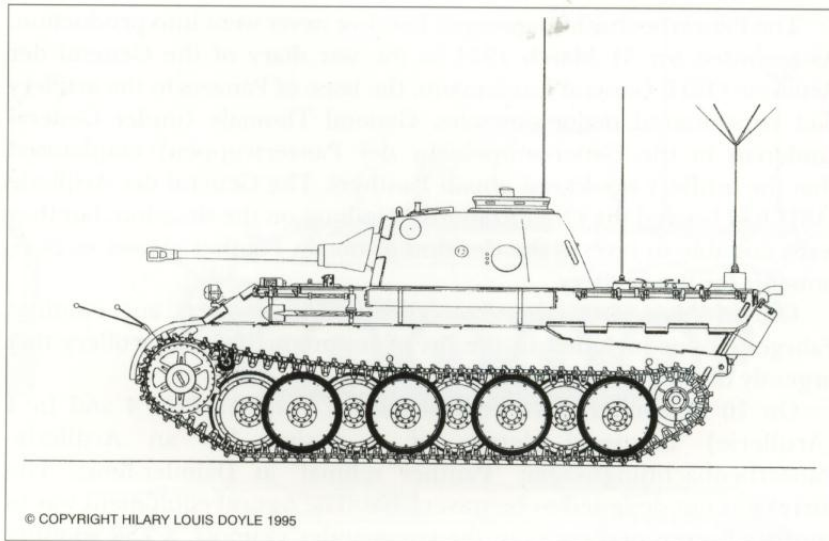
1:76 scale side view drawing of the third proposal for 'Artillerie-Panzer-Beobachtungswagen Fahrgestell Panther' dated 11 November 1942. (Hilary Louis Doyle)
