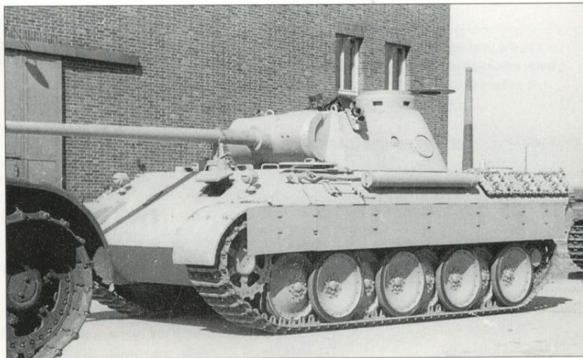
A Panther Ausf.D produced by Henschel in 1943.
