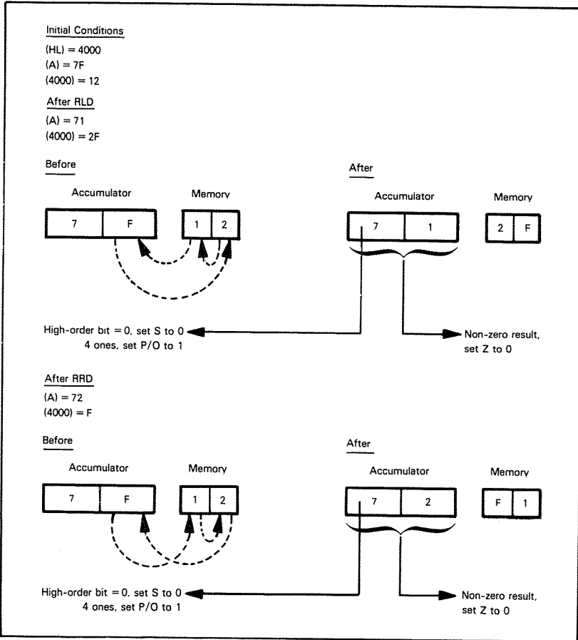
Figure 8-1. Examples of the Z80 Digit Shifts
