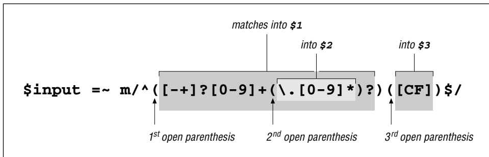
Figure 2-3: Nesting parentheses
