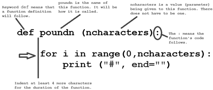
FIGURE 4.1. The syntax of a function definition.
