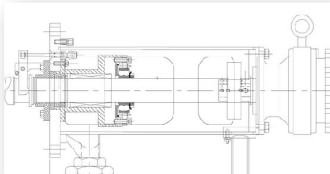
Seal Isolation Unit with Metal on Metal Seating and Single Point Pivot Fork Engagement
