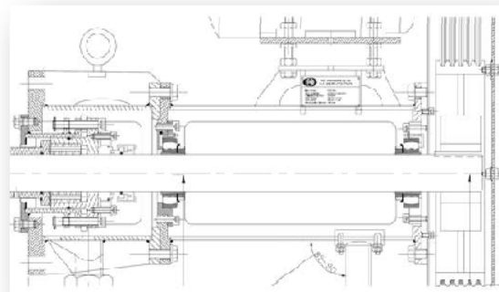
Seal Isolation Unit with Viton Seating and 4 Point clamp Plate
