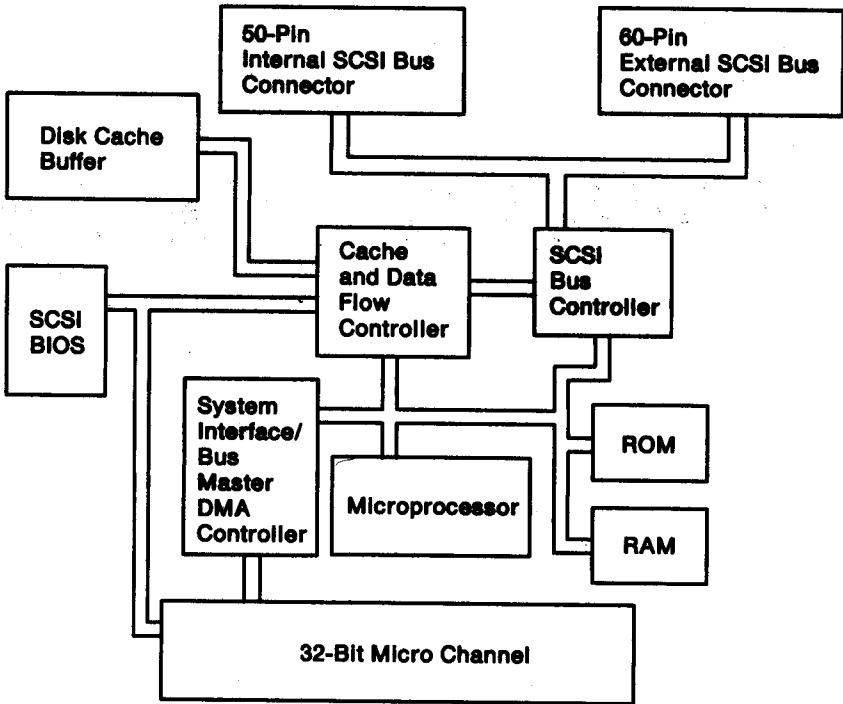
Figure 1. Adapter Block Diagram
