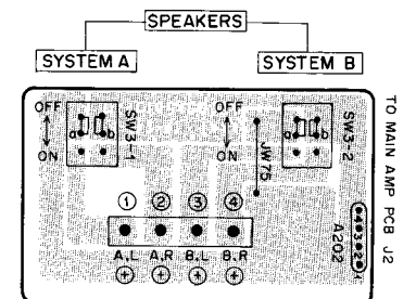
SPEAKER SW PCB A2033A501D [U] A502D [C,A] A503D [E,B,S] A504D [V]
