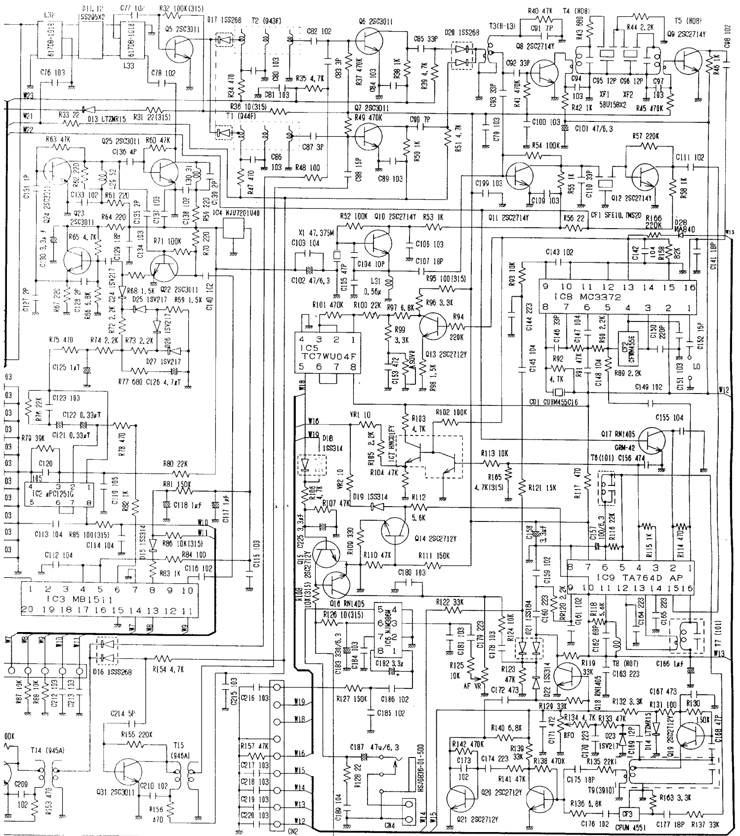
HSC-050 Main Schematic D/M (9/08/09)
