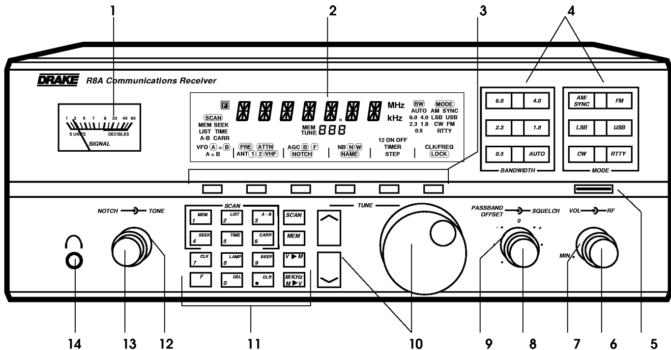
FIGURE 4 FRONT PANEL
