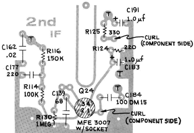
2nd IF AMPLIFIER CIRCUIT BOARD
