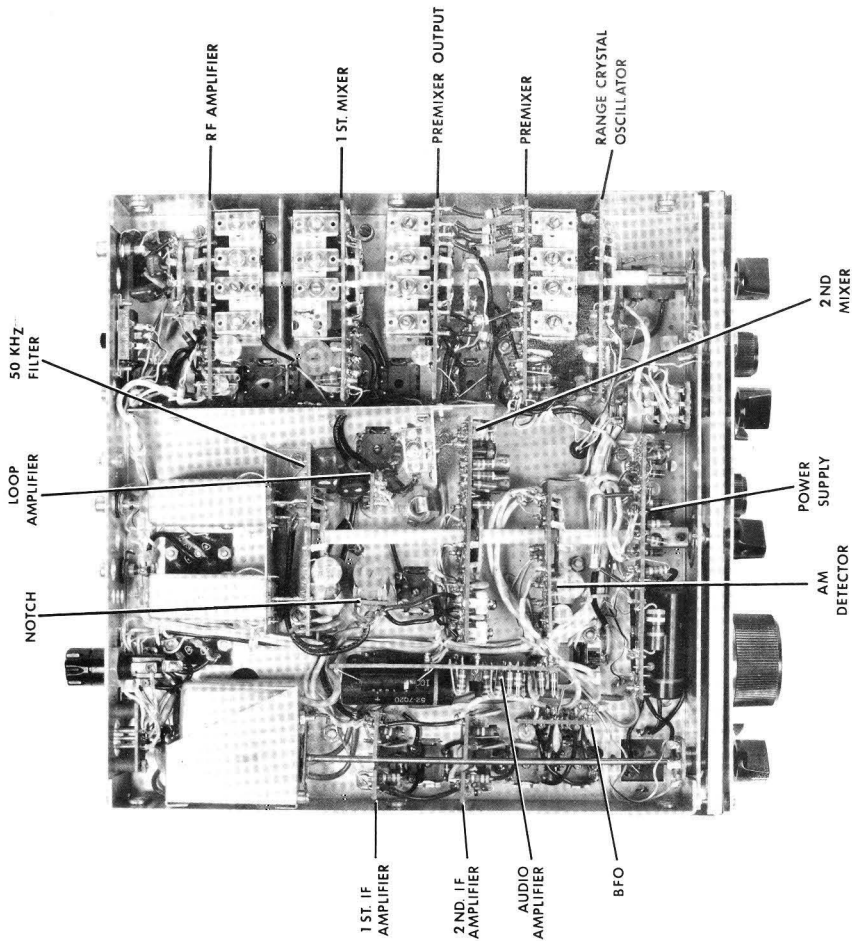
BOTTOM VIEW CIRCUIT BOARD LOCATIONS Figure 20
