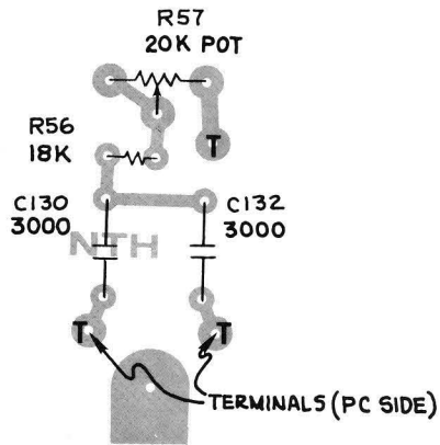
NOTCH FILTER CIRCUIT BOARD Figure 33
