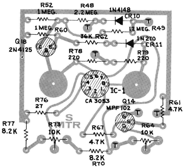
S-METER CIRCUIT BOARD Figure 32
