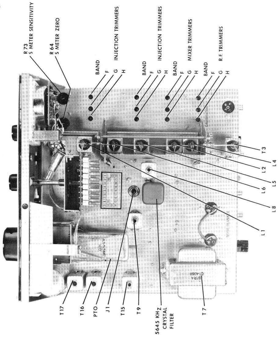
TOP ALIGNMENT ADJUSTMENT POINTS Figure 5
