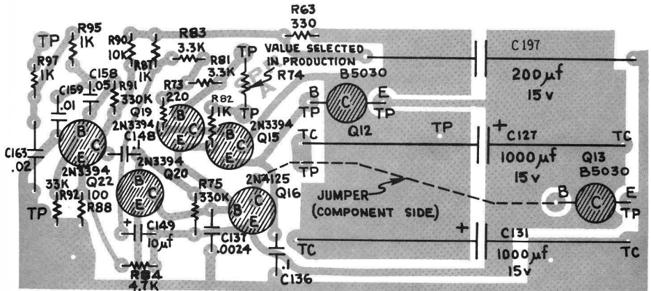
AUDIO AMPLIFIER CIRCUIT BOARD
