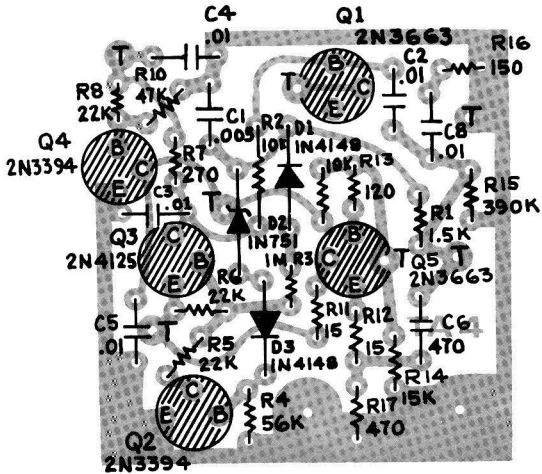
TA-4 CIRCUIT BOARD
