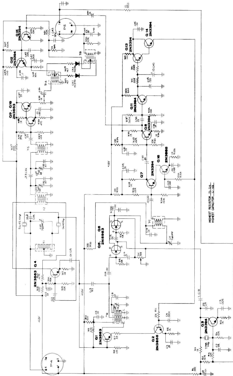
5-NB SCHEMATIC DIAGRAM Figure 11
