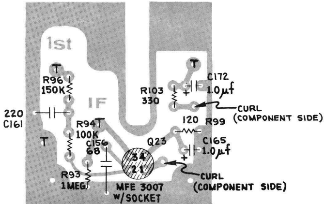
1st IF AMPLIFIER CIRCUIT BOARD
