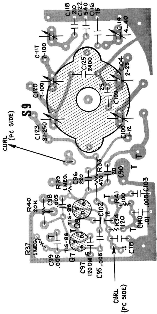
1st MIXER CIRCUIT BOARD Figure 28
