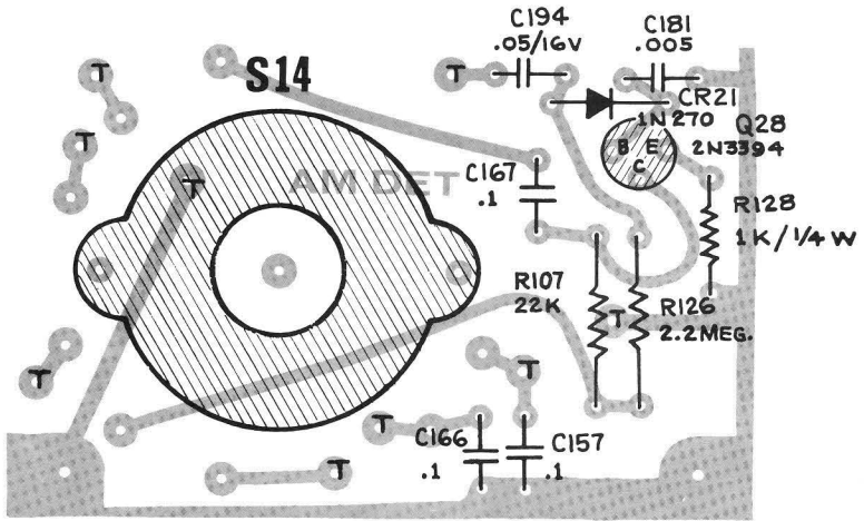
AM DETECTOR CIRCUIT BOARD
