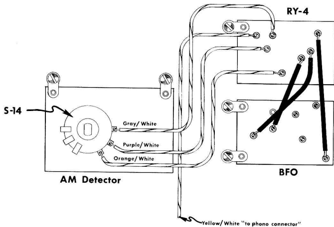
RY-4 PICTORIAL WIRING DIAGRAM Figure 13
