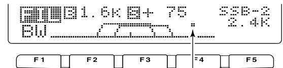
Appears when passband is shifted. *By pushing [PBTC] for 1 sec., the shifted value returns to the default setting, and the “dot” disappears.
