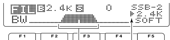
Reverses Appears While pushing [F1 BW], rotate the tuning dial to set passband width.
