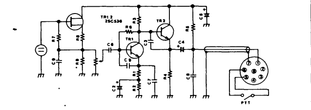
Schematic diagram of IC-SM6
