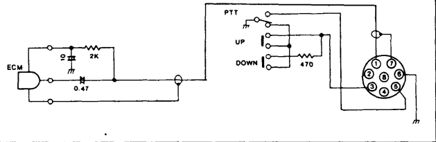
Schematic diagram of IC-SM6
