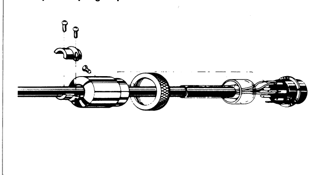
Microphone plug exploded view
