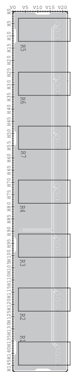
• VR-C BOARD (TOP VIEW)
