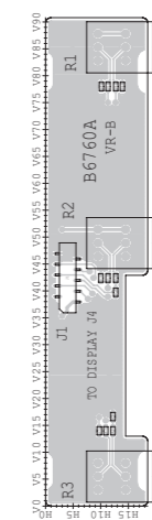
• VR-B BOARD (TOP VIEW)
