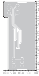
• PBT BOARD (BOTTOM VIEW)
