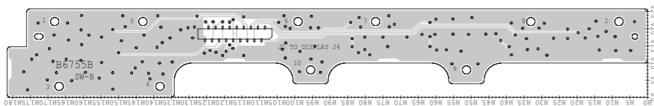
• SW-B BOARD (BOTTOM VIEW)
