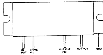
SC-1019 IC1 (VHF RF POWER AMP)
