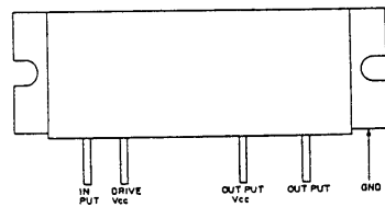
SC-1027 IC2 (UHF RF POWER AMP)
