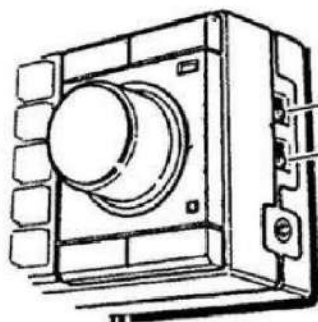
㉒ DIMMER SWITCH ㉓ LOCK SWITCH
