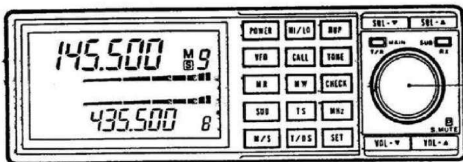
⑩ TUNING CONTROL
