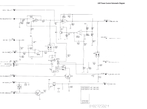
MP Power Amplifier Schematic Diagram
