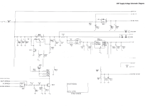
MP Supply Voltage Schematic Diagram
