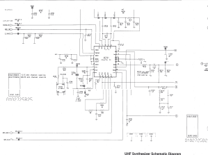
MP Synthesizer Schematic Diagram
