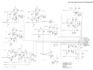
MP Control Bus Controller Schematic Diagram
