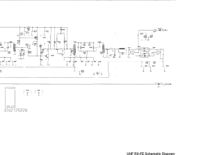
MP PLL Schematic Diagram
