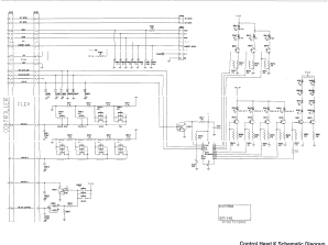
Control Panel Schematic Diagram
