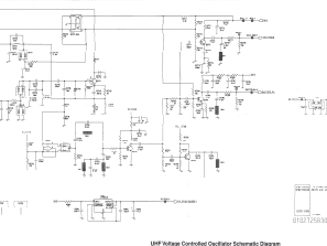
MP Voltage Control Schematic Diagram
