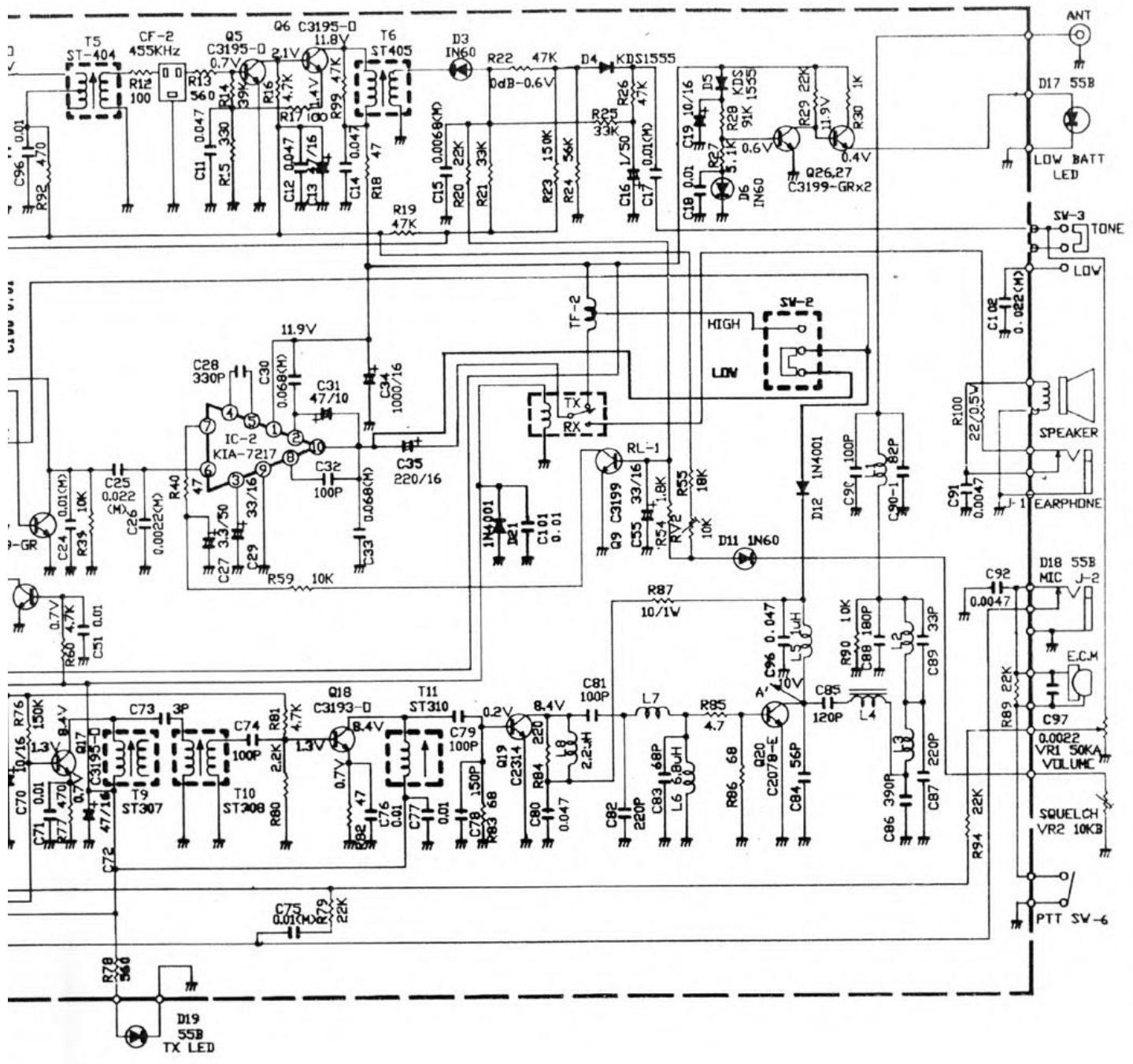
SCHEMATIC DIAGRAM PRO-200
