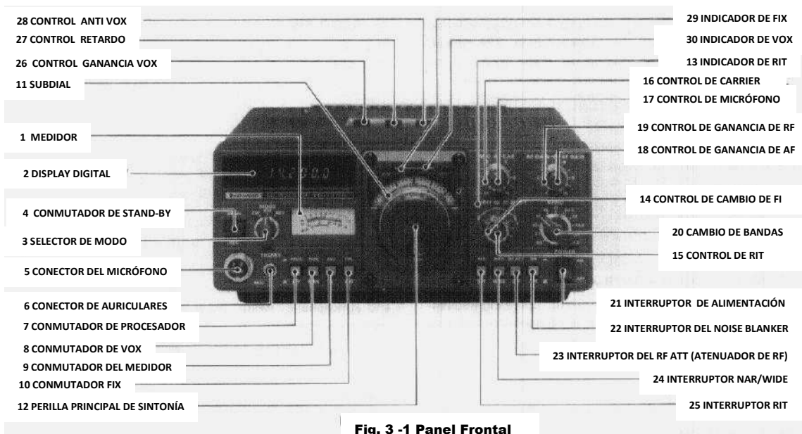
Fig. 3 -1 Panel Frontal
