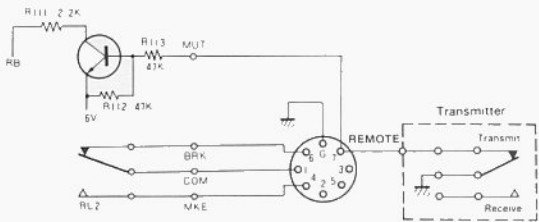
Fig. 5-1 Remote Terminal
