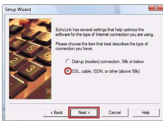
Figure 8-11 Type of Connection
