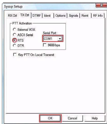
Figure 8-38 Sysop Setup Window: TX Ctrl Tab
