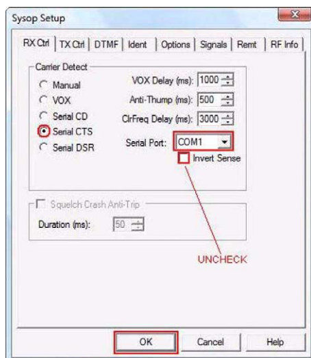
Figure 8-37 Sysop Setup Window: RX Ctrl Tab
