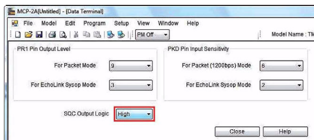
Figure 8-46 MCP-2A Data Terminal Window: SQC Output Logic
